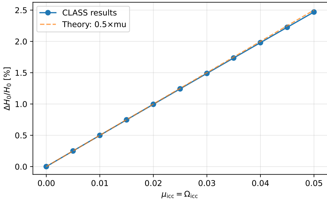
ICC-R2: H0 dependence on Omega_icc
