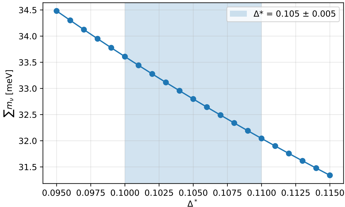
ICC-R2: Neutrino mass sum vs. defect parameter
