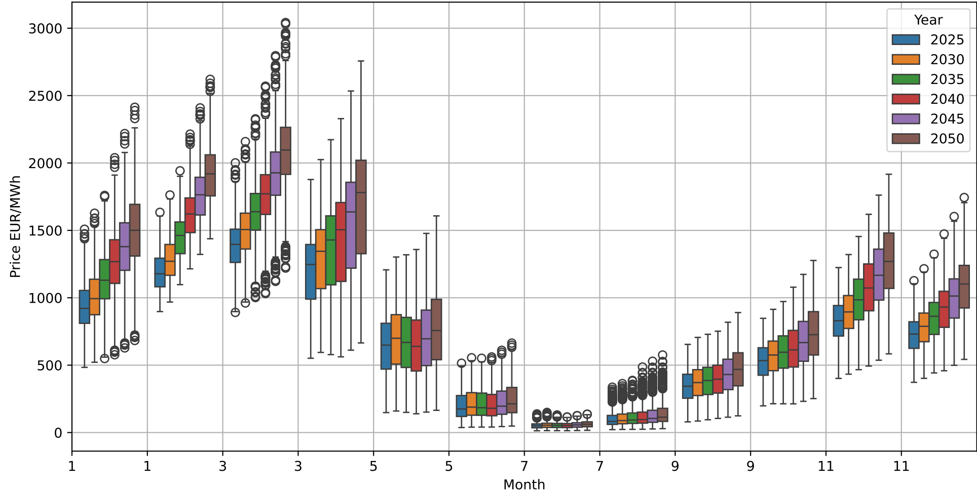
Monthly Distribution of Electricity low prices (EUR/MWh)
