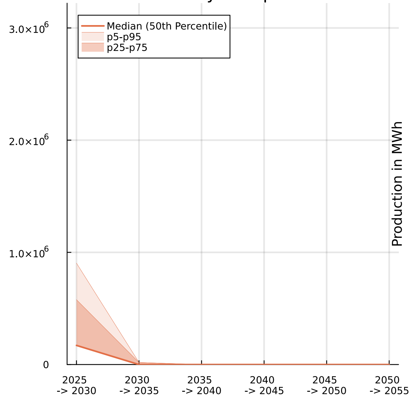
Yearly CHP prod
