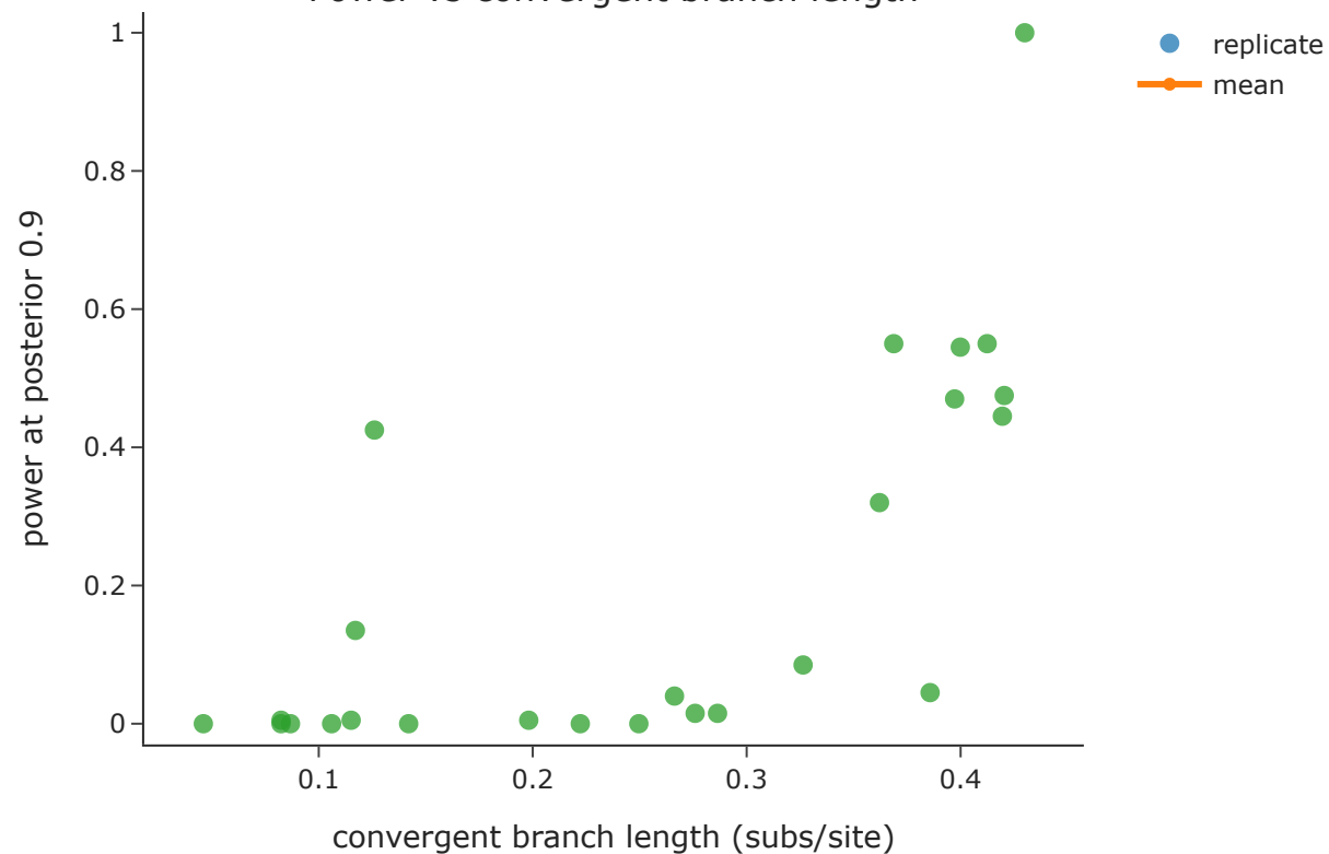
Power vs convergent branch length
