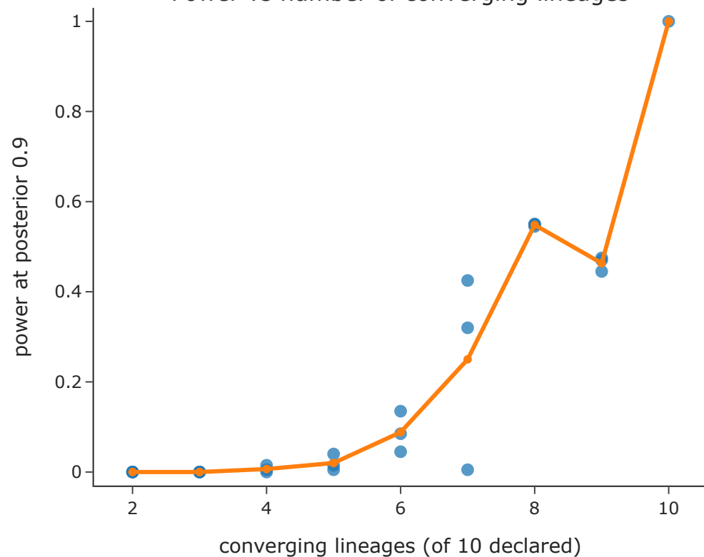
Power vs number of converging lineages
