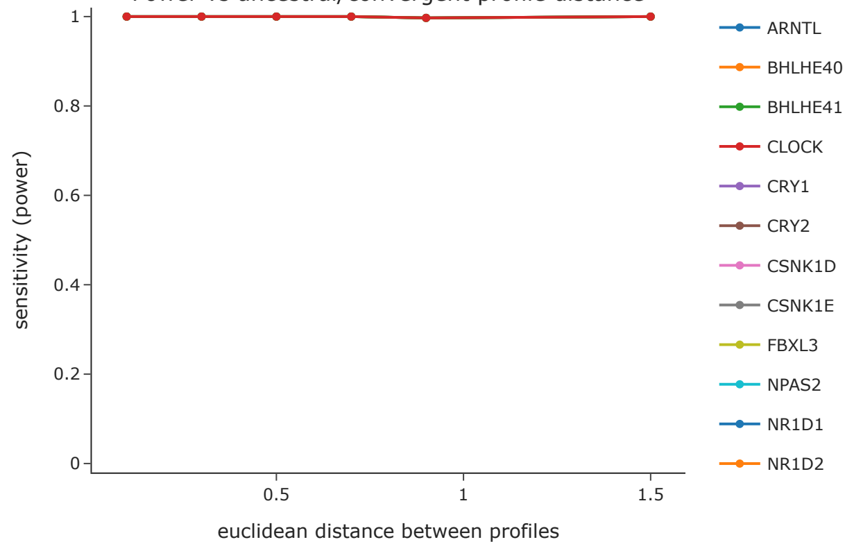
Power vs ancestral/convergent profile distance
