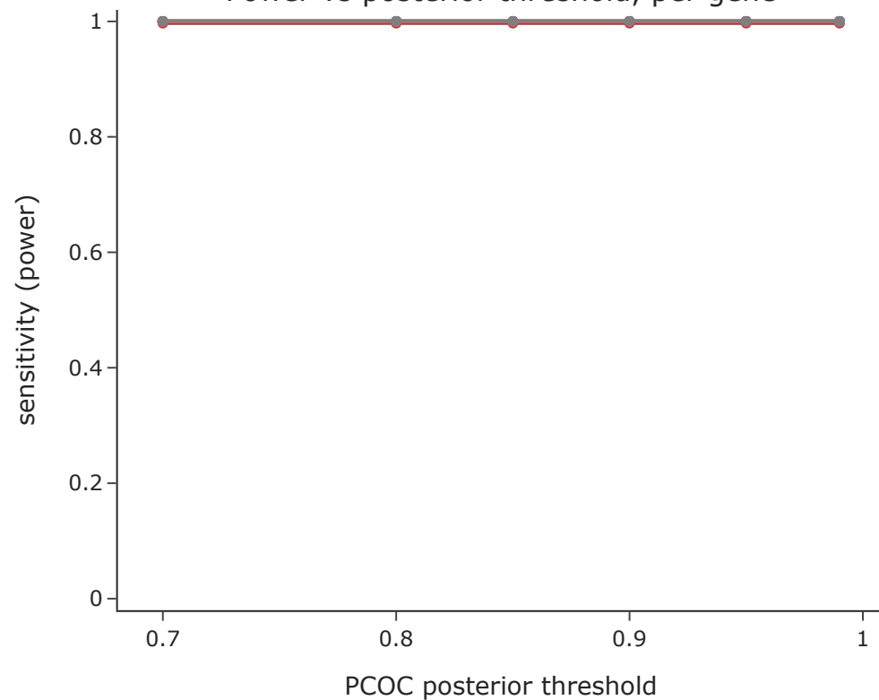
Power vs posterior threshold, per gene
