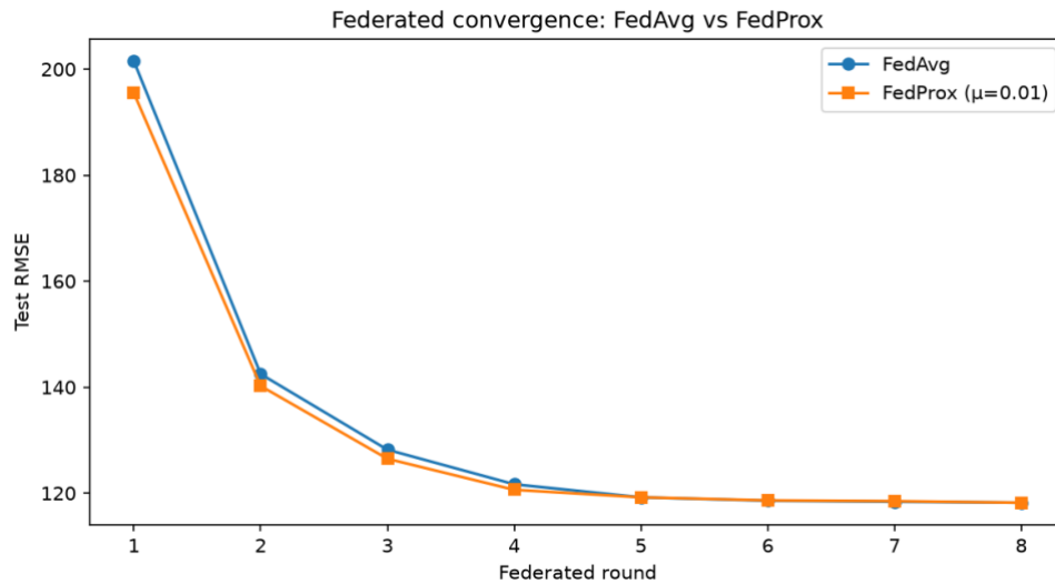
Figure 4.8: Federated learning convergence — FedAvg vs FedProx ( \mu = 0.01 ). Both strategies converge to equivalent final RMSE ( \sim 118 ) after eight rounds. FedProx converges marginally faster in rounds 2–4, consistent with its proximal regularisation reducing early client drift under the geographic non-IID partition.
