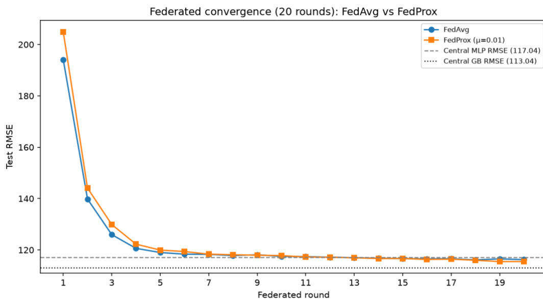
Figure 4.13: Federated convergence over 20 rounds (FedAvg vs FedProx) with centralised MLP and Gradient Boosting RMSE reference lines.
