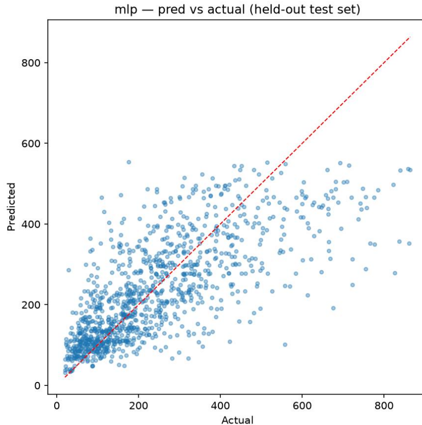
Figure 4.7b: Predicted versus actual primary energy intensity for the centralised MLP (held-out test set, R^2 = 0.528 ). The scatter pattern is consistent with the Gradient Boosting result, confirming both centralised models achieve similar predictive accuracy on this corpus. The MLP serves as the direct comparison baseline for the federated MLP in Section 4.3.
