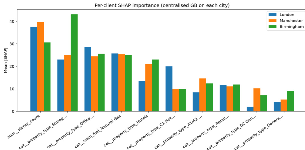
Figure 4.14: Per-client SHAP comparison (centralised Gradient Boosting applied to each city). Bars show mean |SHAP| for the top features by city.
