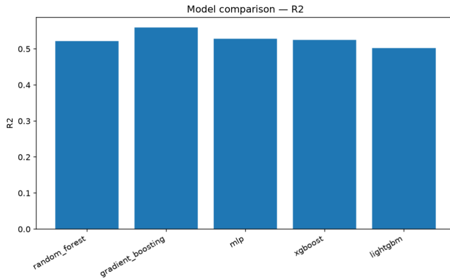
Figure 4.6: Centralised baseline R^2 comparison. Absolute accuracy remains moderate ( R^2 \approx 0.50 – 0.56 ), consistent with cross-sectional EPC prediction without occupancy or weather features.
