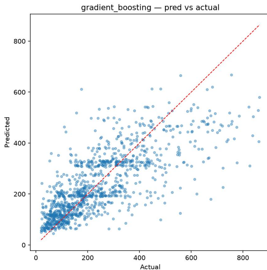
Figure 4.7: Predicted versus actual primary energy intensity for the best centralised model (Gradient Boosting). Absolute errors increase at higher intensities.
