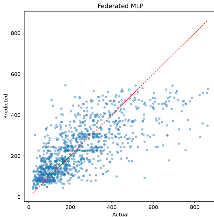
Figure 4.9: Predicted versus actual primary energy intensity for the federated MLP. Residual magnitude pattern is similar to the centralised tree model, with slightly higher MAE.
