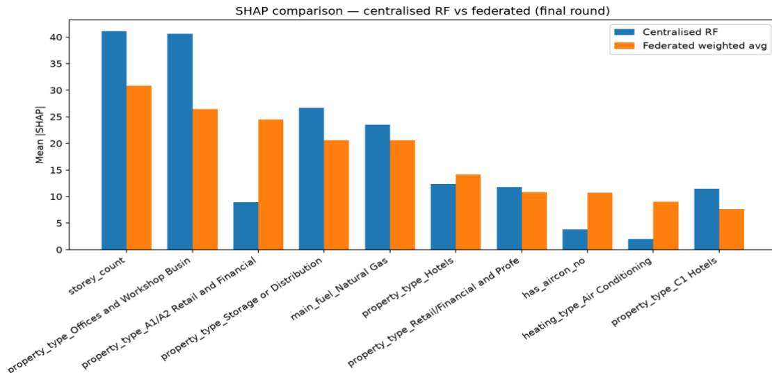
Figure 4.10: SHAP comparison — Centralised RF vs Federated weighted average. Blue = centralised; orange = federated. Feature rankings show strong agreement across training regimes.
