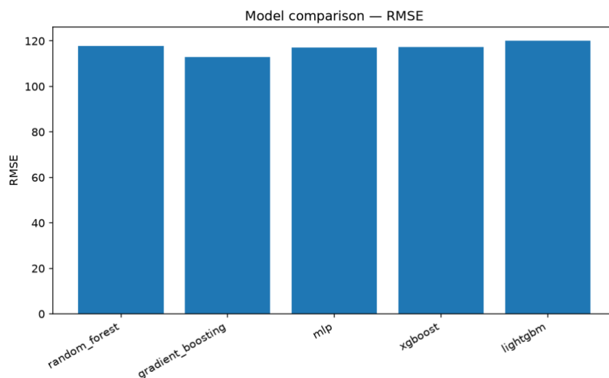
Figure 4.5: Centralised baseline RMSE comparison. Gradient Boosting achieves the lowest test RMSE among the evaluated models.
