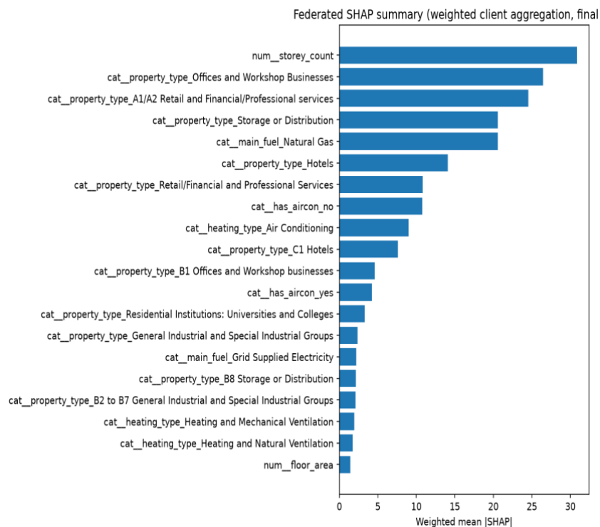
Figure 4.11: Federated SHAP summary (weighted client aggregation). num_storey_count dominates, followed by commercial property type indicators and fuel type.
