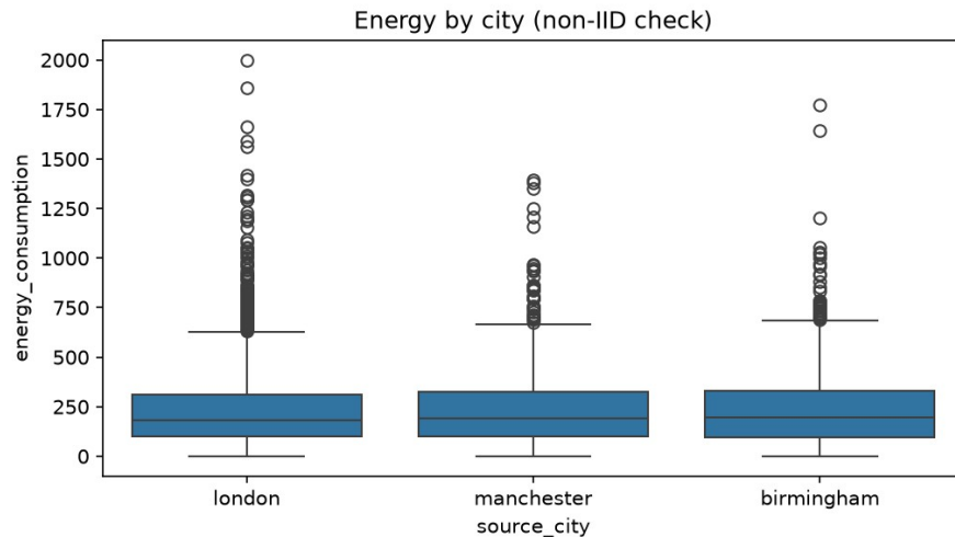
Figure 4.3: Energy distribution by client city (boxplot, non-IID check). Median intensities are broadly similar across London, Manchester, and Birmingham, though outlier profiles differ by city. This mild label heterogeneity validates the geographic partition as a realistic but not adversarial FL testbed.
