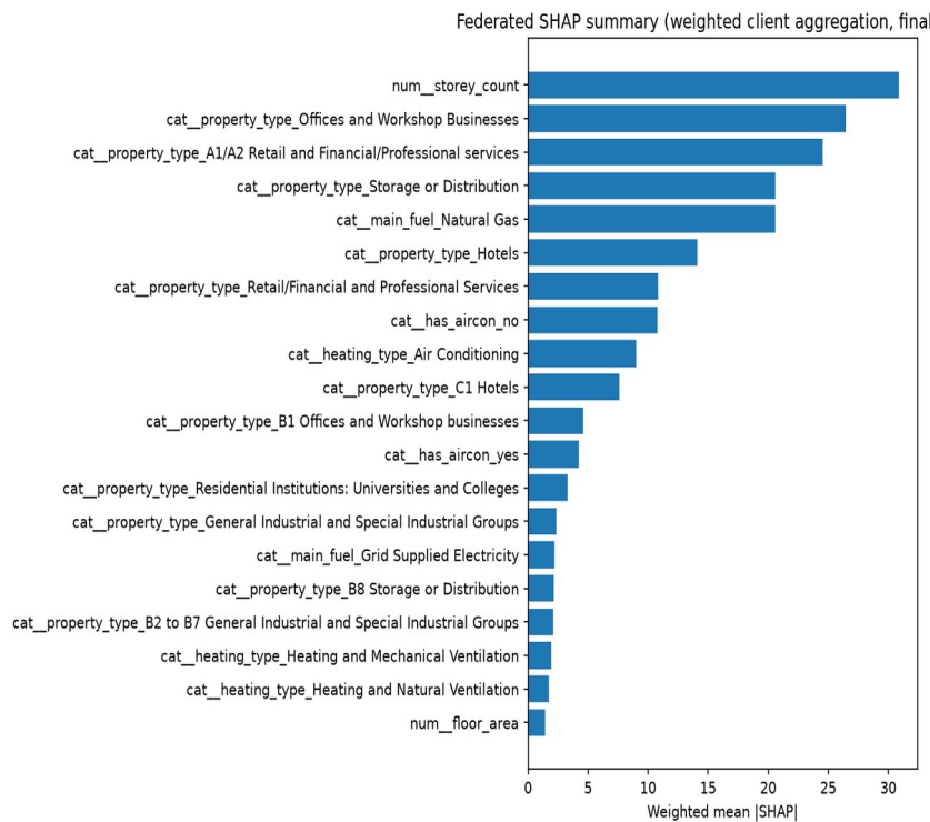
Figure 4.11: Federated SHAP summary (weighted client aggregation). num__storey_count dominates, followed by commercial property type indicators and fuel type.
