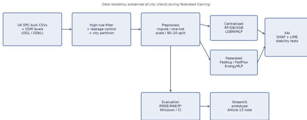
Figure 3.1 — PP-XAI end-to-end experimental pipeline
