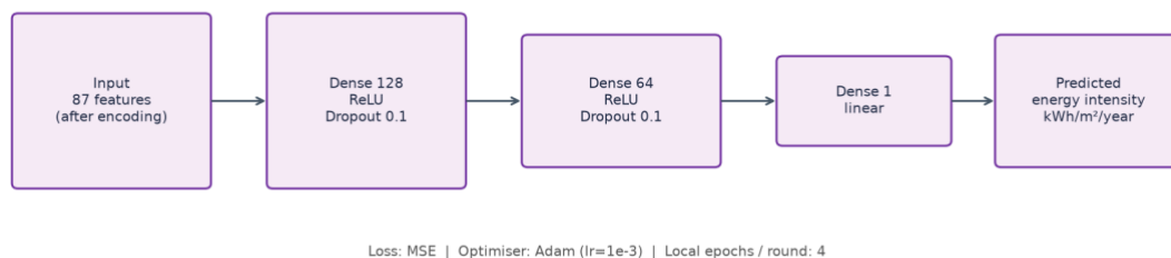
Figure 3.3: EnergyMLP architecture (federated and central neural baseline).
