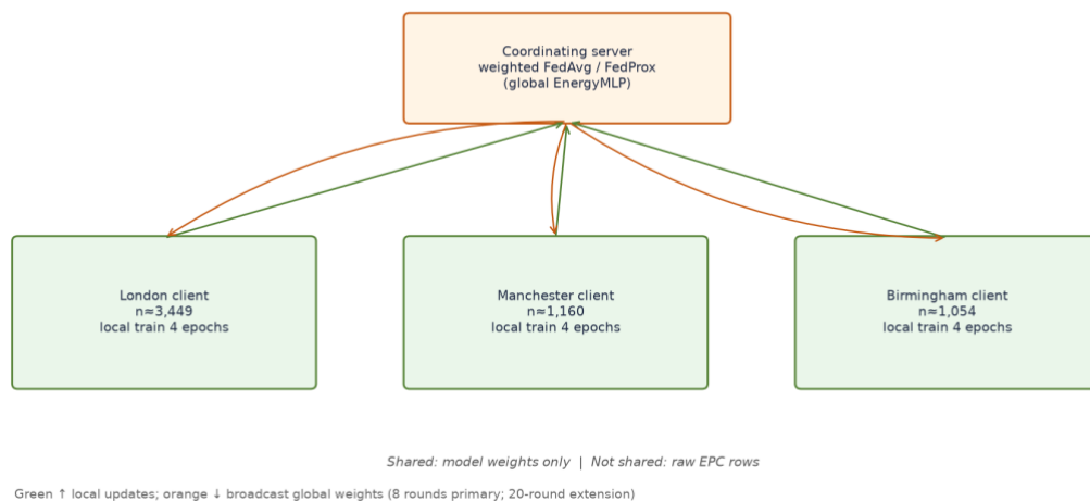
Figure 3.2 — Federated Averaging architecture (three geographic clients)
