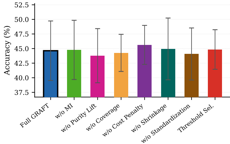
Chameleon-F
