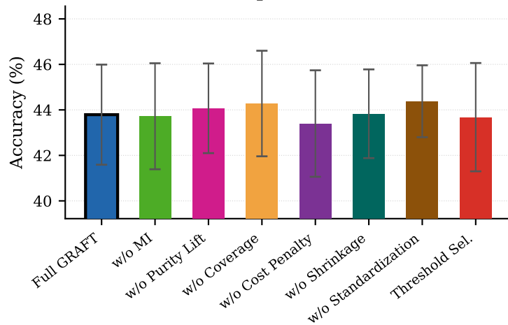
Squirrel-F
