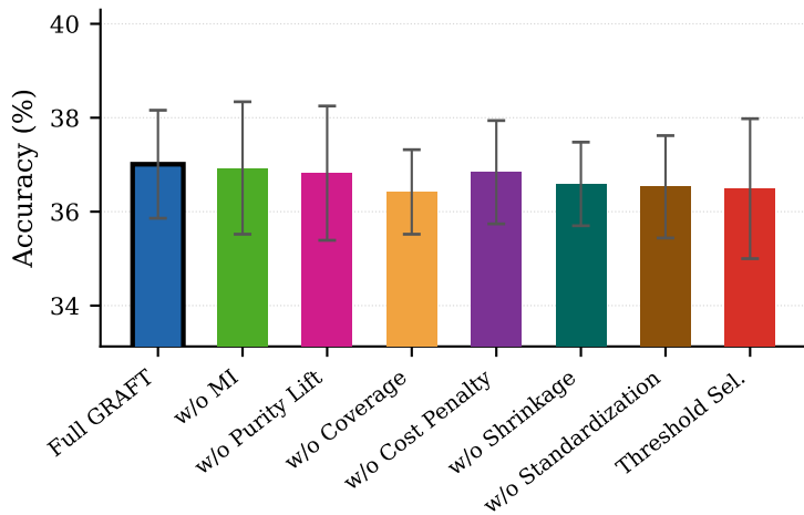
ACTOR
