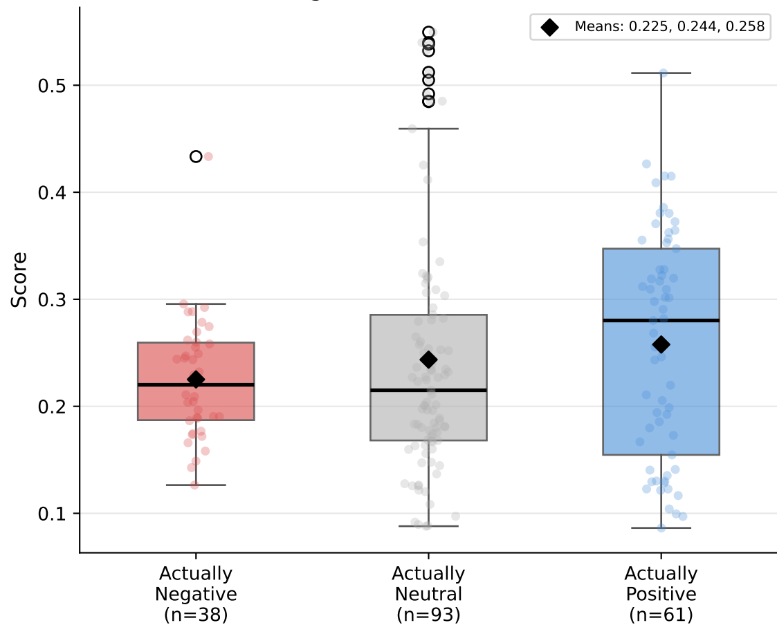
Negative Sentiment Score
