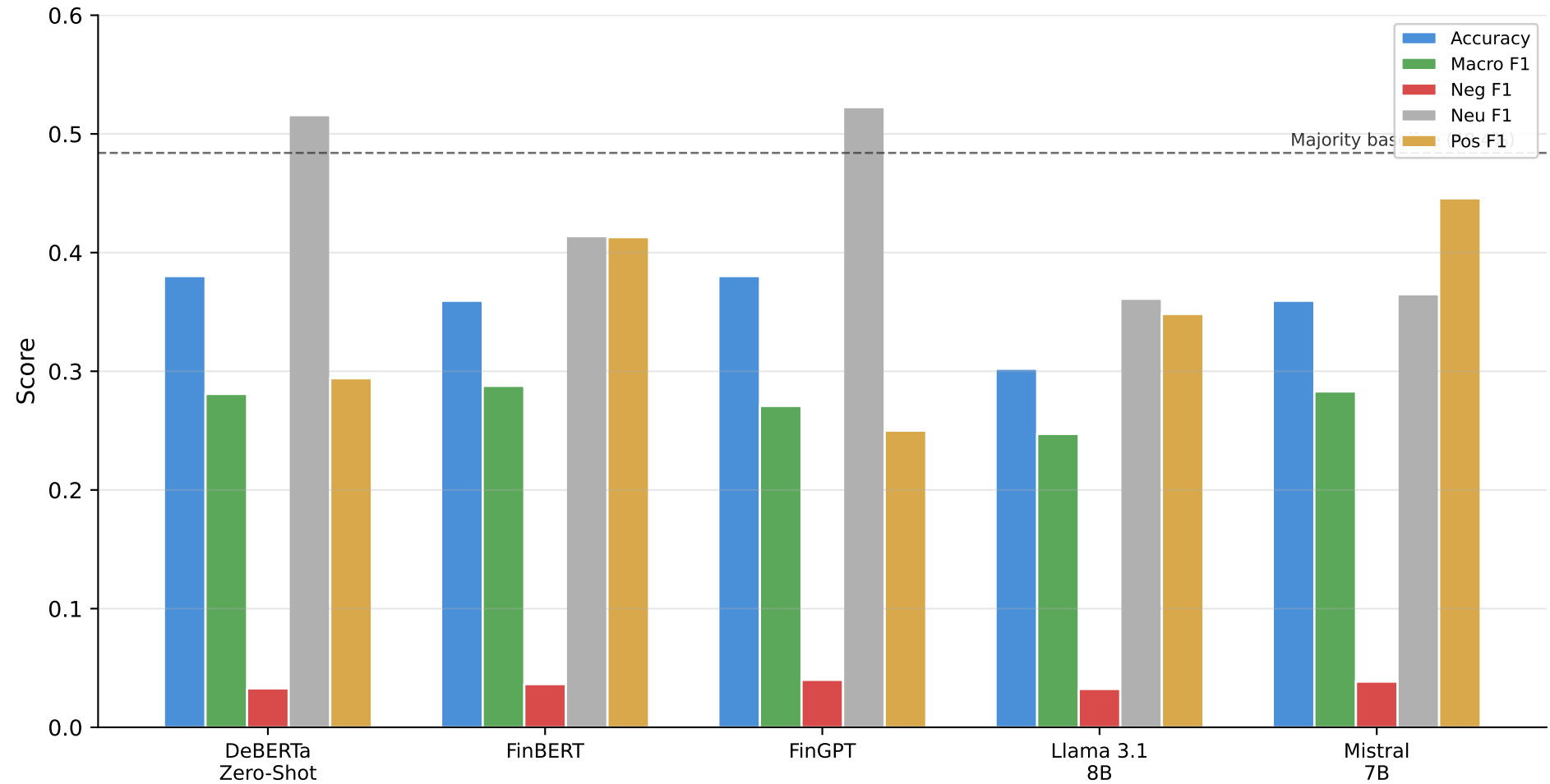
Model Comparison on Holdout Set (192 cases)
