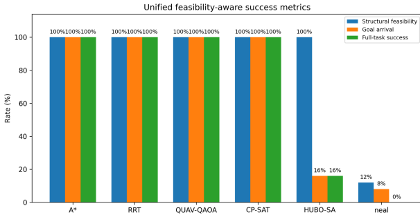
Figure 2: Unified feasibility-aware success metrics. The exact CP-SAT run certifies a full-success optimum. neal has nonzero feasibility and goal-arrival rates separately, but zero full-task success.
