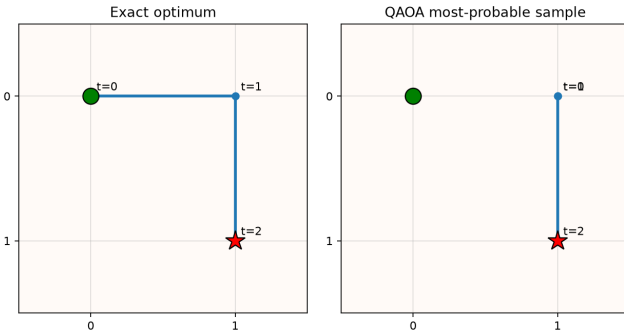
Fig. 4: Reduced Qiskit decoded-path check. The exact feasible optimum reaches the target through a valid two-step path. The most-probable direct-QAOA sample reaches the target but violates hard feasibility constraints, demonstrating why bitstring decoding must be reported separately from expected energy.
