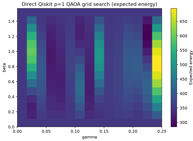
Fig. 3: Direct Qiskit p = 1 QAOA grid search on the reduced 2 \times 2, L = 3 instance. The heatmap shows expected energy over the sampled (\gamma, \beta) grid. This is a reduced gate-based compatibility check, not a full-instance solver.
