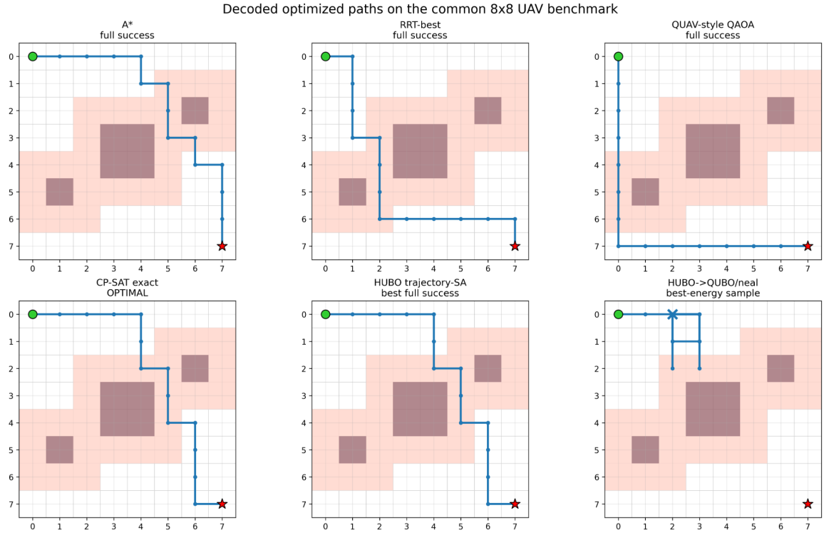
Figure 2: Decoded optimized paths on the common 8 \times 8 , L = 20 benchmark. Dark cells are obstacles, light cells are obstacle-buffer cells, the green circle is the start, and the red star is the target. The CP-SAT path is globally optimal for the hard-feasible native-HUBO soft objective. The neal path is the best-energy decoded QUBO sample; the cross marks its terminal cell and illustrates a quadratization/sampling failure mode because the path does not reach the target.
