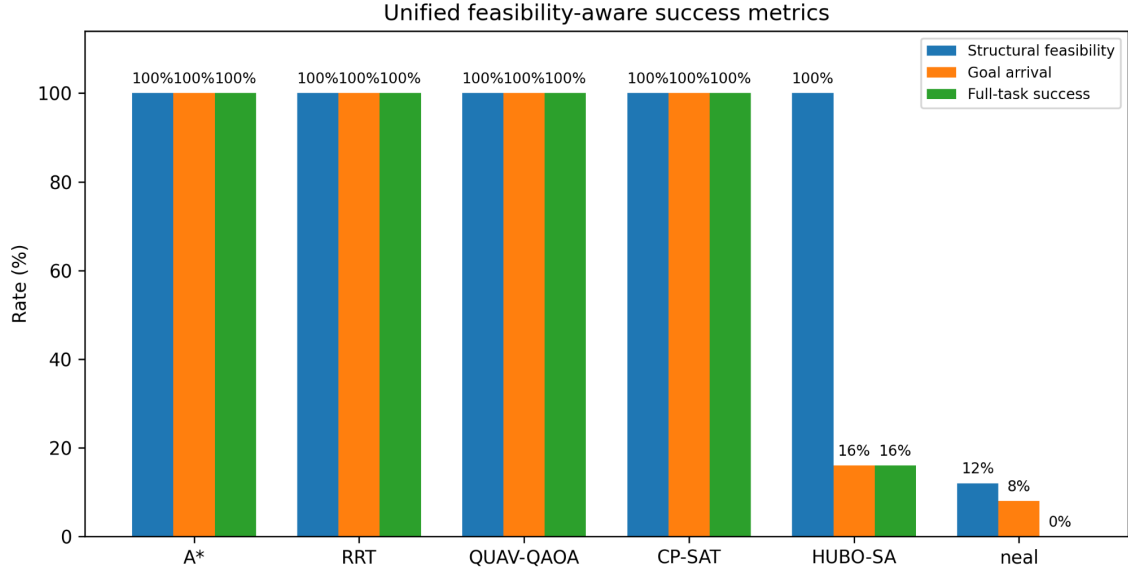
Figure 1: Unified feasibility-aware success metrics. Exact CP-SAT certifies a full-success optimum. The neal sampler has nonzero structural-feasibility and goal-arrival rates separately, but zero full-task success.
