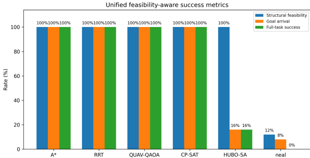
Figure 2: Feasibility-aware success metrics. CP-SAT certifies a full-success optimum; neal has nonzero separate feasibility and goal-arrival rates but no full-task success.
