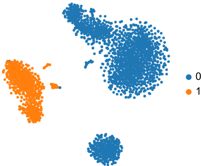
TSNE - kmeans_k2
