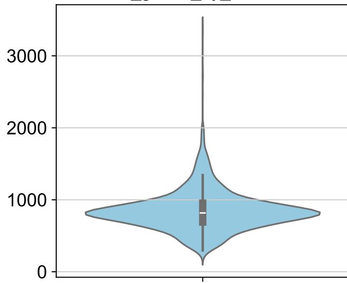
n_genes_by_counts
