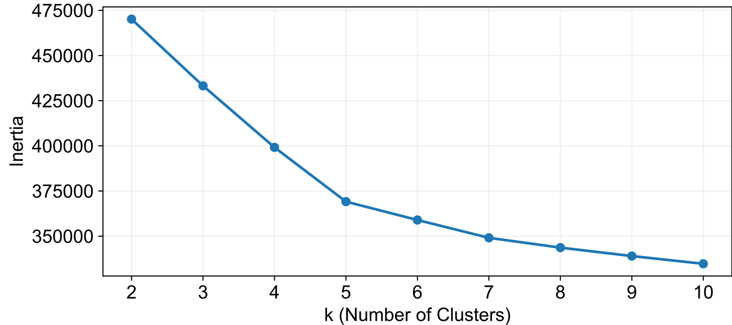
K-Means Elbow Plot
