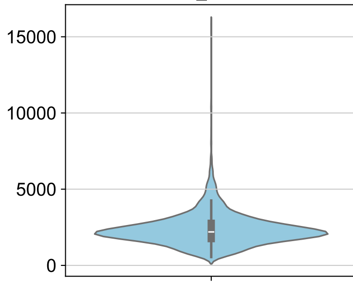
total_counts
