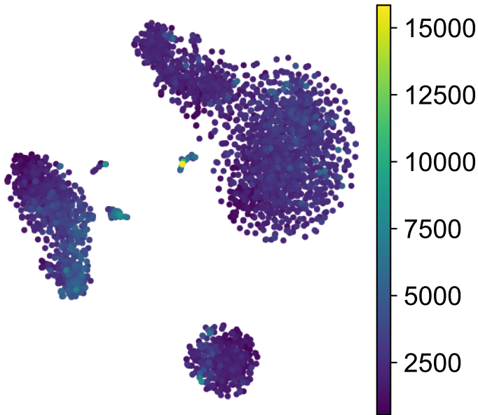
TSNE - total_counts
