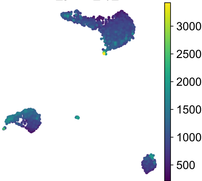
UMAP - n_genes_by_counts
