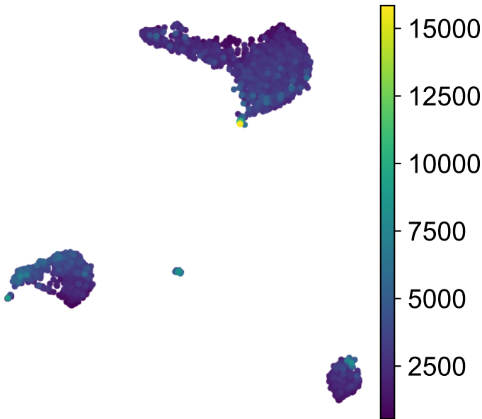
UMAP - total_counts
