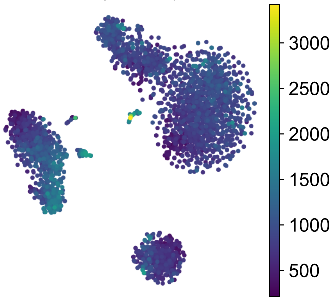
TSNE - n_genes_by_counts
