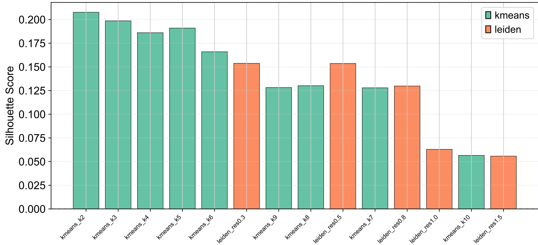
Silhouette Score Comparison Across Clustering Methods
