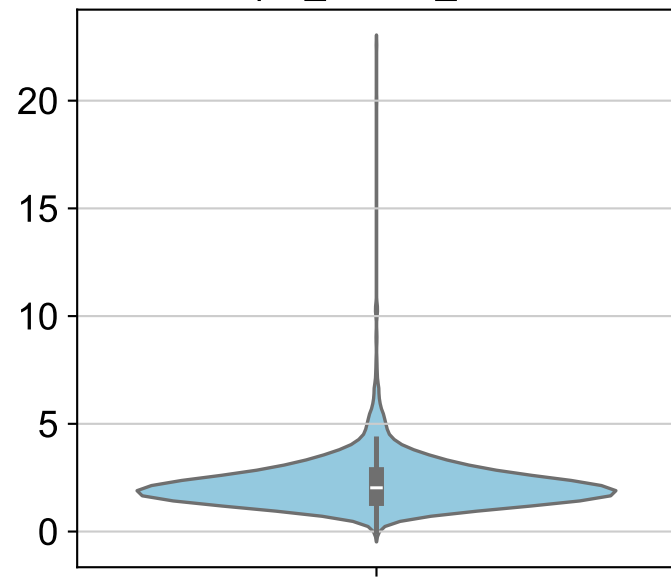
pct_counts_mt
