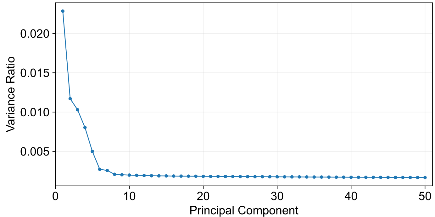
PCA Elbow / Scree Plot
