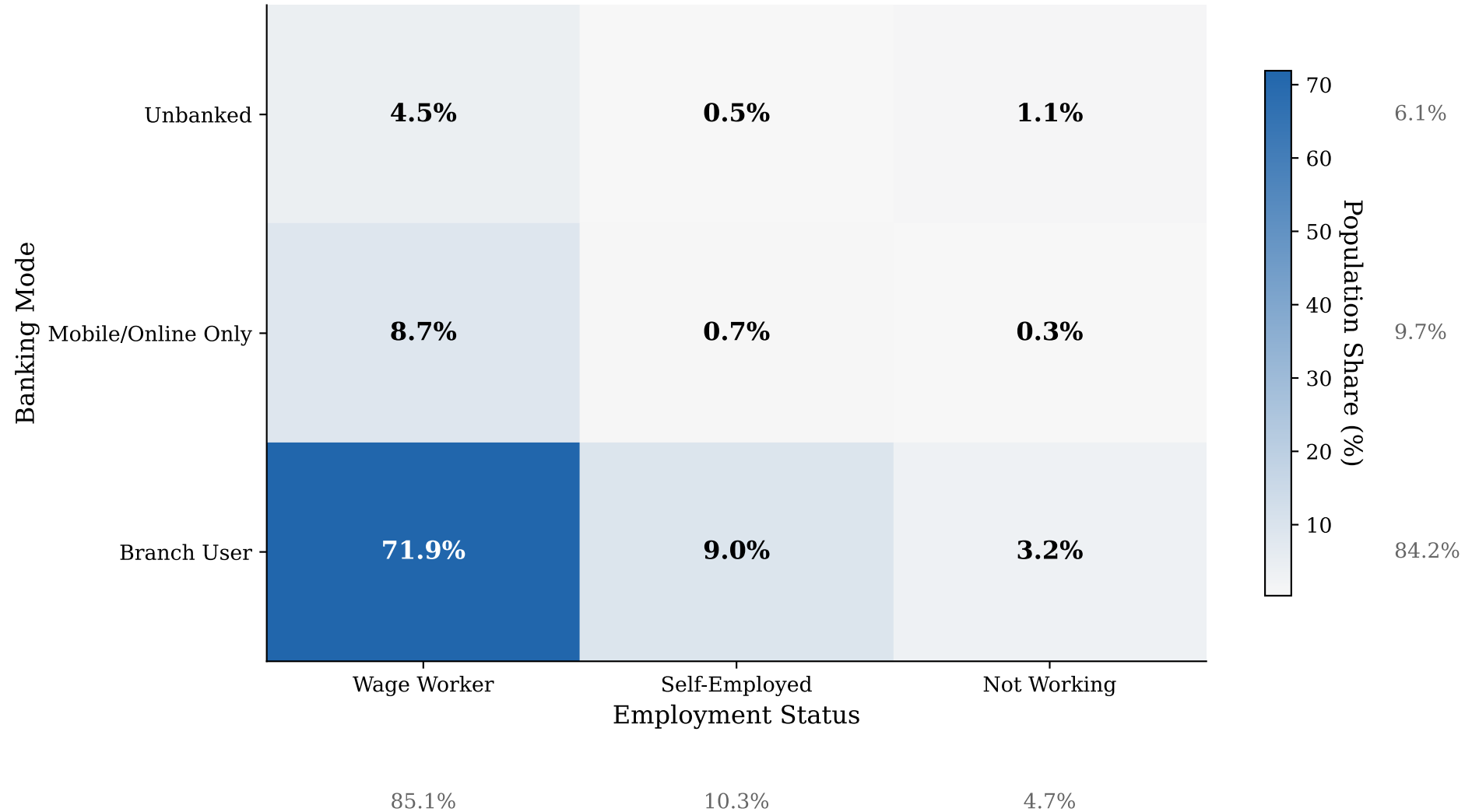
Joint Distribution of Banking Mode and Employment Status
