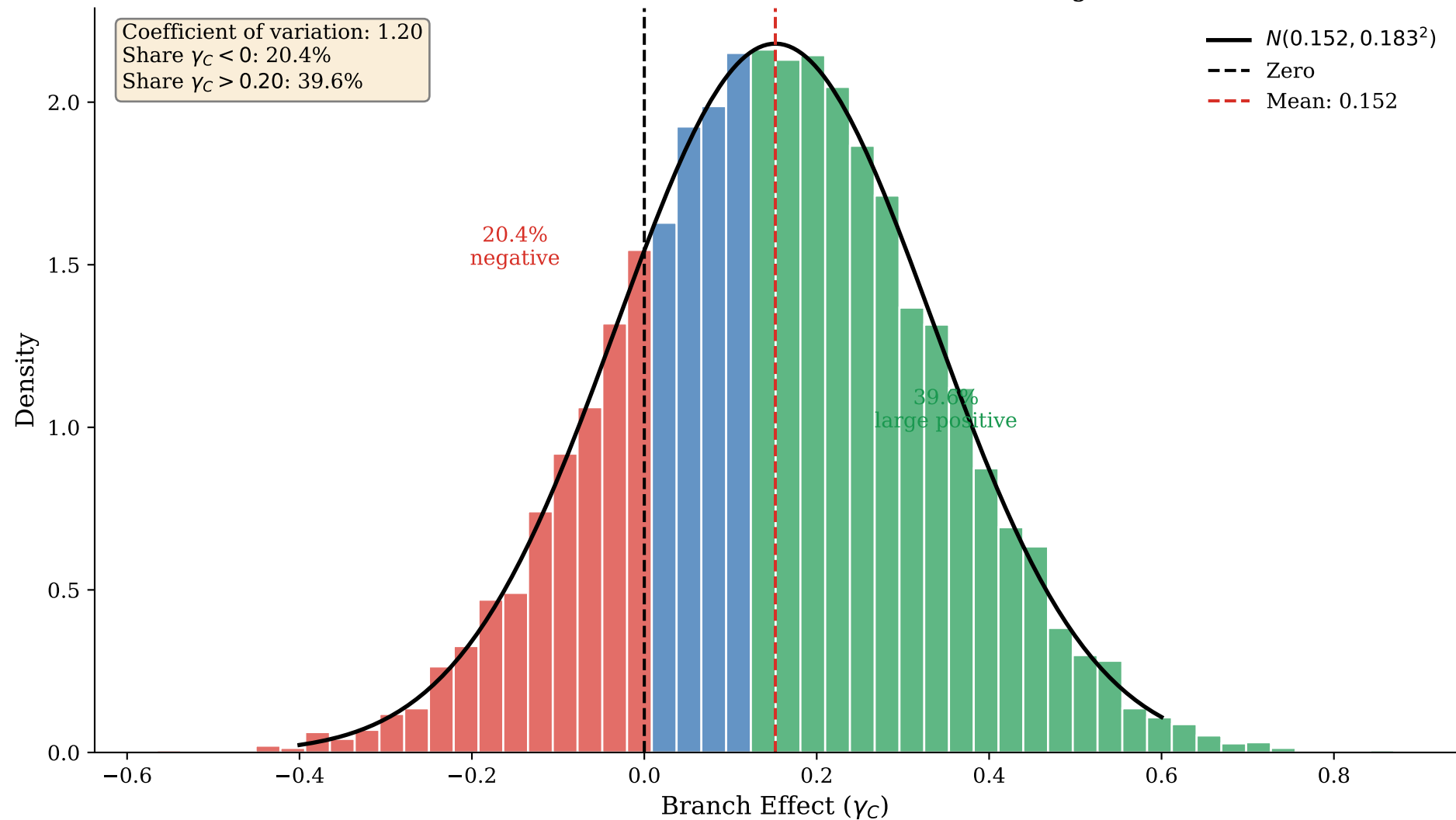
Distribution of Random Coefficients (Mixed Logit)
