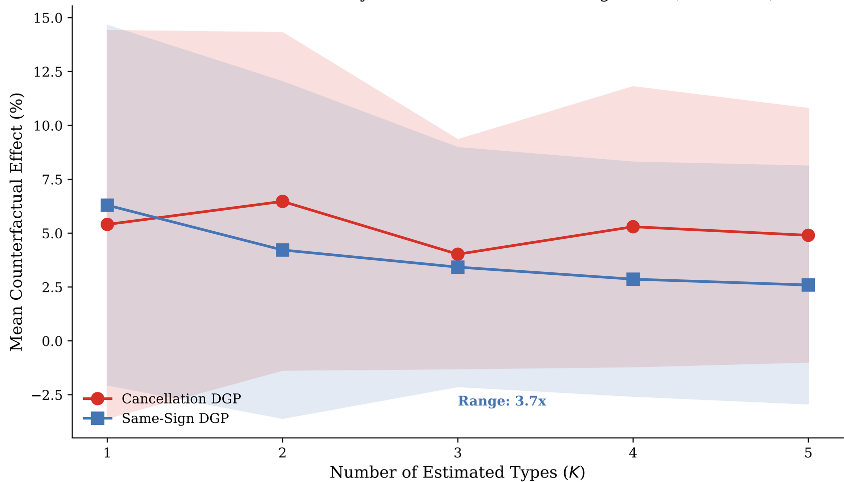
Counterfactual Sensitivity: Cancellation vs. Same-Sign DGP (N=10,000)
