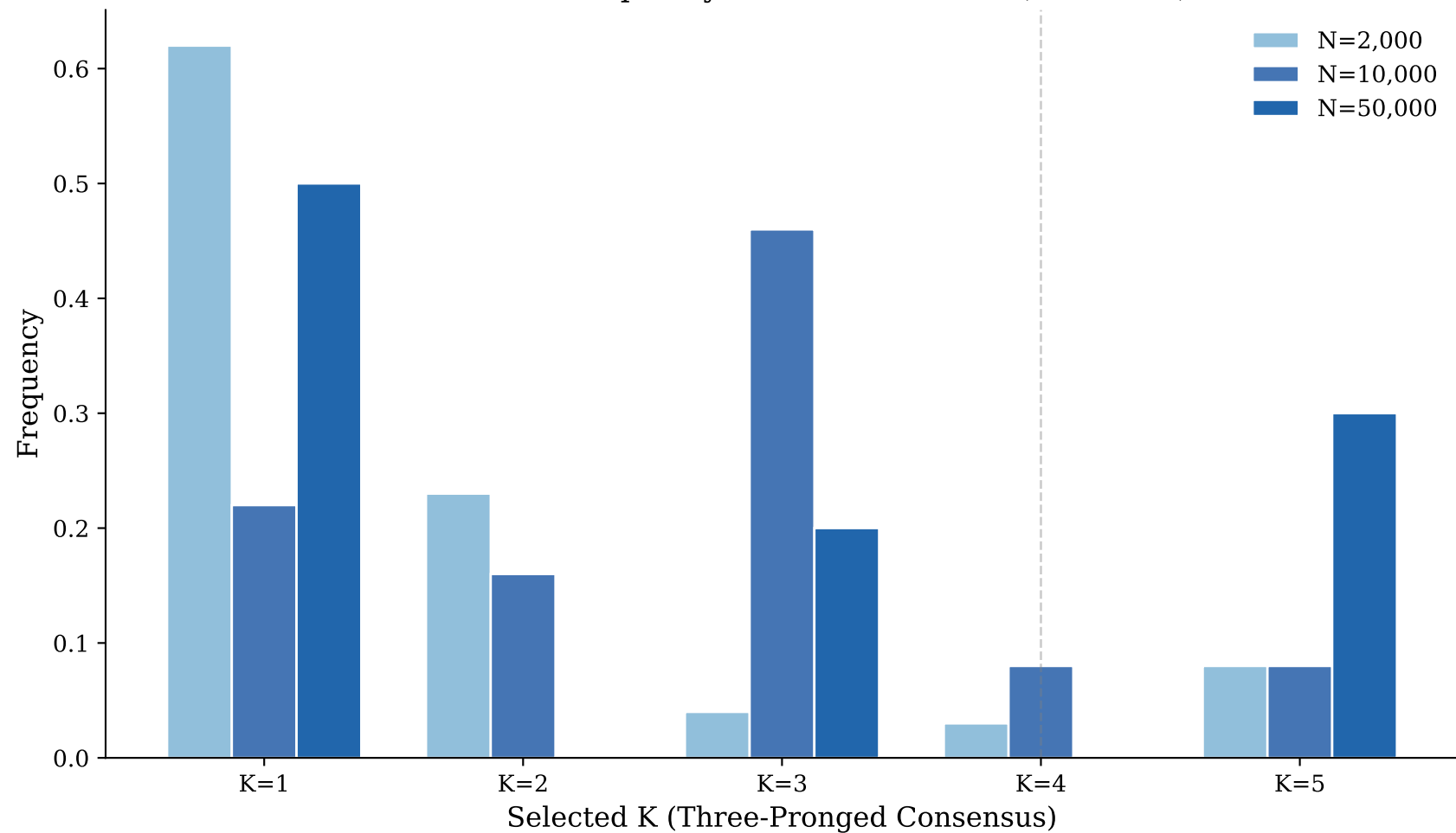
K Selection Frequency: Cancellation DGP (True K=4)
