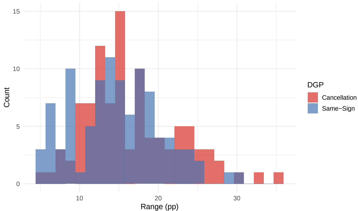
Distribution of CF Range Across K
