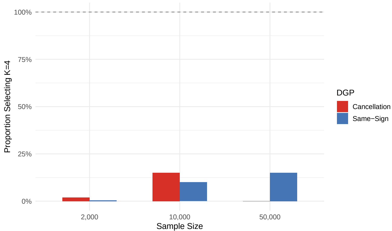
BIC Selection Accuracy (True K=4)
