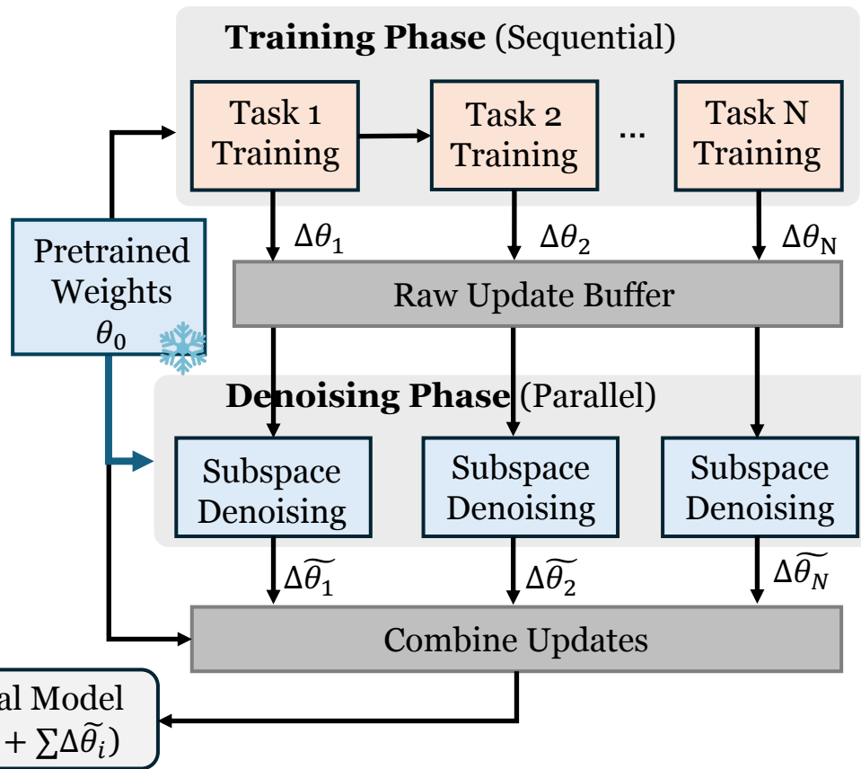
(b) SLoRA-Post
