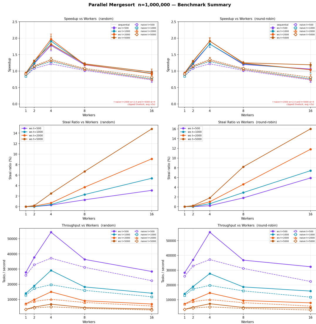
Figure 3: Mergesort benchmarks
