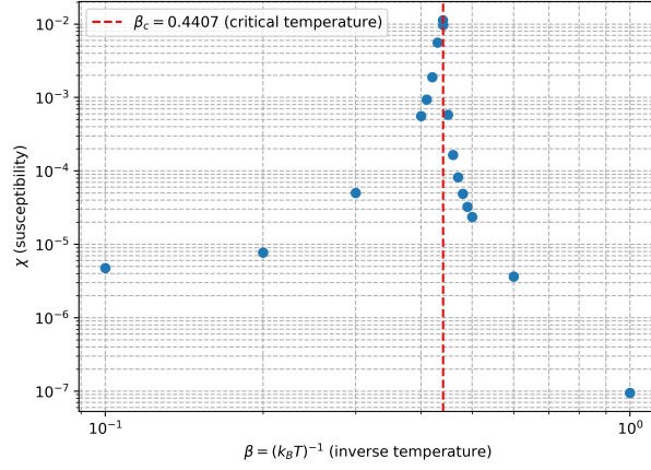
Figure 6: Susceptibility versus inverse temperature \beta using Wolff updates. Points show the equilibrium susceptibility computed via fluctuation-dissipation theorem. The red dashed line indicates the critical value \beta_c .
