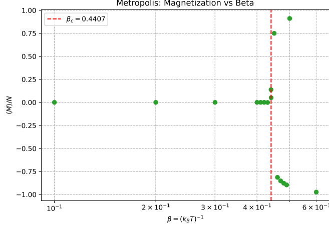
Figure 3: Magnetization versus inverse temperature \beta using Metropolis updates. Points show the equilibrium average magnetization. The red dashed line indicates the critical value \beta_c .
