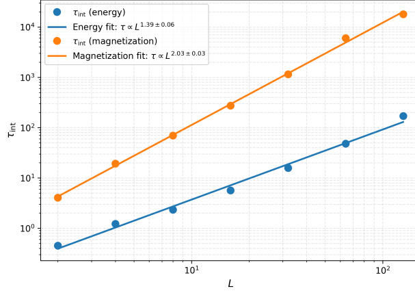
Figure 8: Finite-size scaling of integrated autocorrelation time \tau versus system size L at criticality \beta_c \approx 0.4407 for energy (blue) and magnetization (orange) using Metropolis updates.
