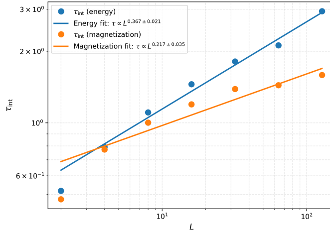
Figure 9: Finite-size scaling of integrated autocorrelation time \tau versus system size L at criticality \beta_c \approx 0.4407 for energy (blue) and magnetization (orange) using Wolff updates.
