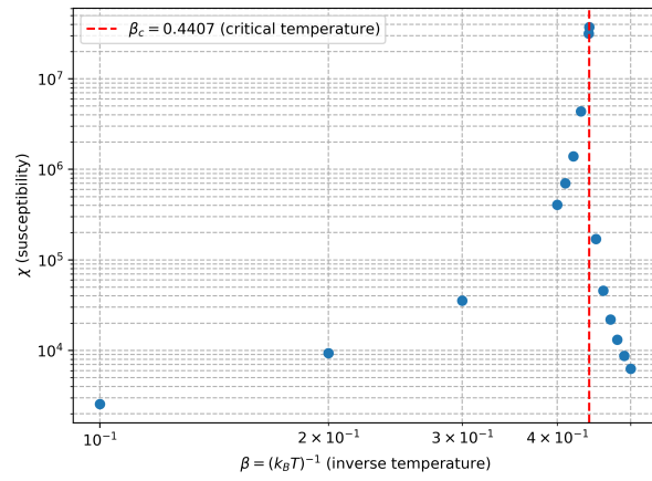
Figure 5: Susceptibility versus inverse temperature \beta using Metropolis updates. Points show the equilibrium susceptibility computed via fluctuation-dissipation theorem.
