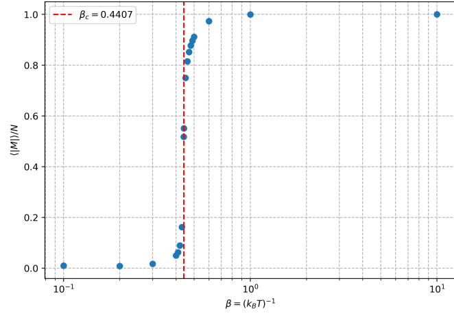
Figure 4: Magnetization versus inverse temperature \beta using Wolff updates. Points show the equilibrium average magnetization.
