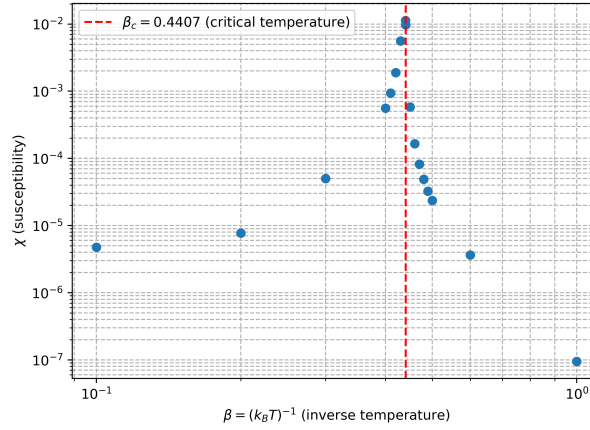
Figure 6: Susceptibility versus inverse temperature \beta using Wolff updates. Points show the equilibrium susceptibility computed via fluctuation-dissipation theorem.
