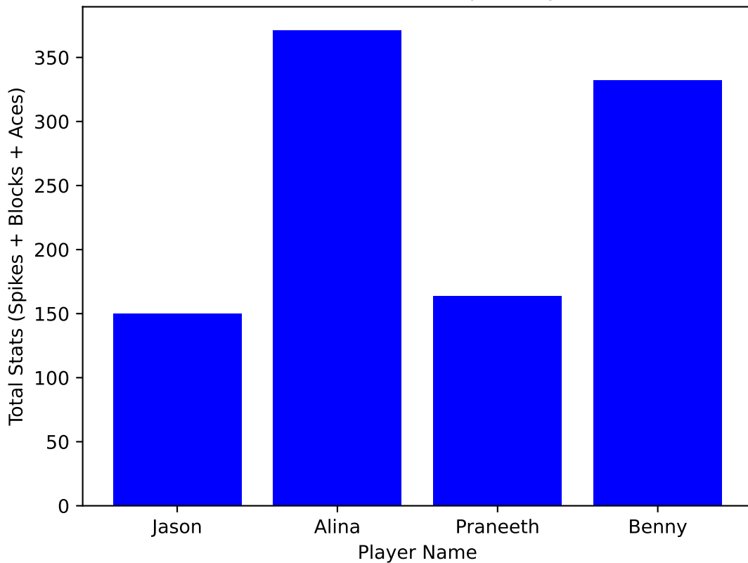
Overall MVP Points per Player
