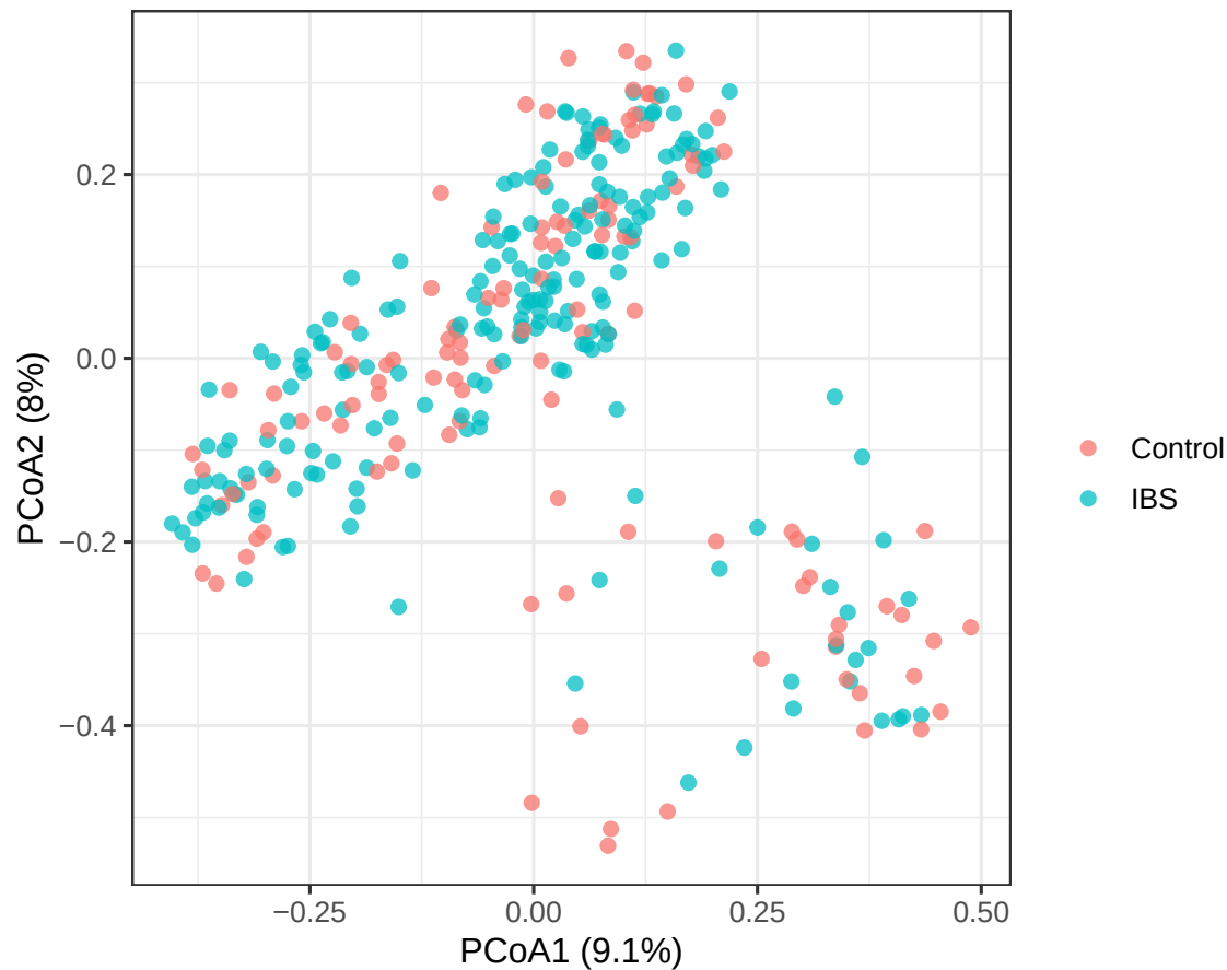
PCoA of species-level MetaPhlAn profiles
