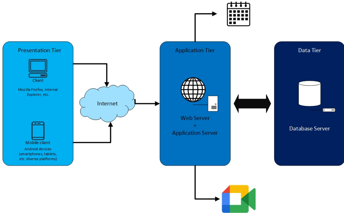
Figure 2: System Architecture
