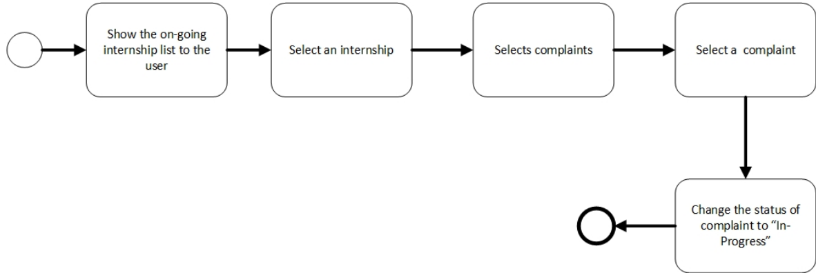
Figure 13: Receiving Complaint by a University State Chart
