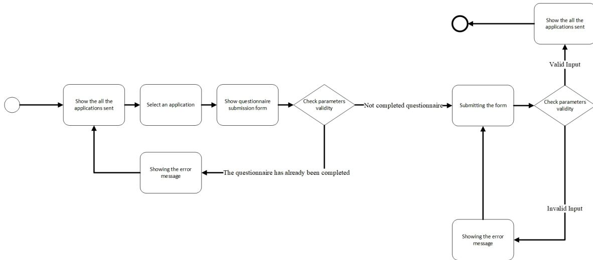
Figure 9: Answering a Questionnaire by a Student State Chart
