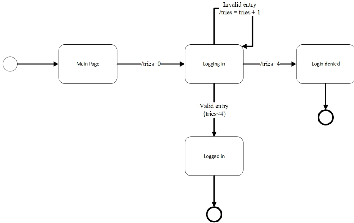
Figure 2: Login State Chart
