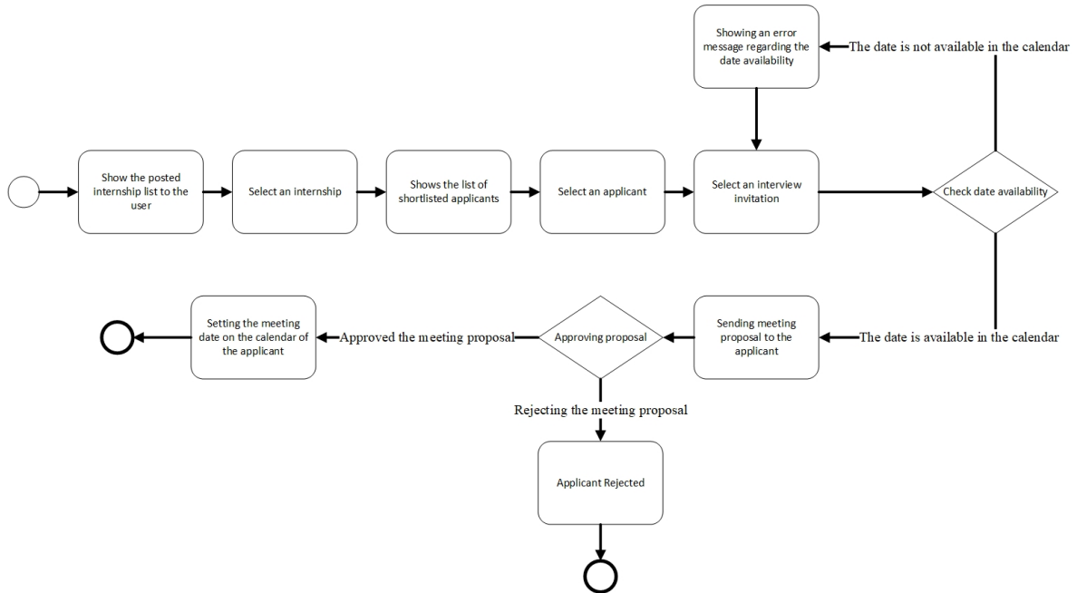
Figure 7: Scheduling Interview by a Company State Chart
