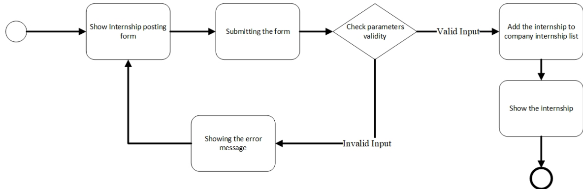
Figure 3: Internship Posting State Chart
