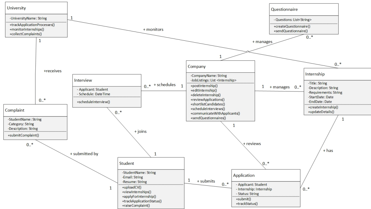
Figure 1: Class Diagram
