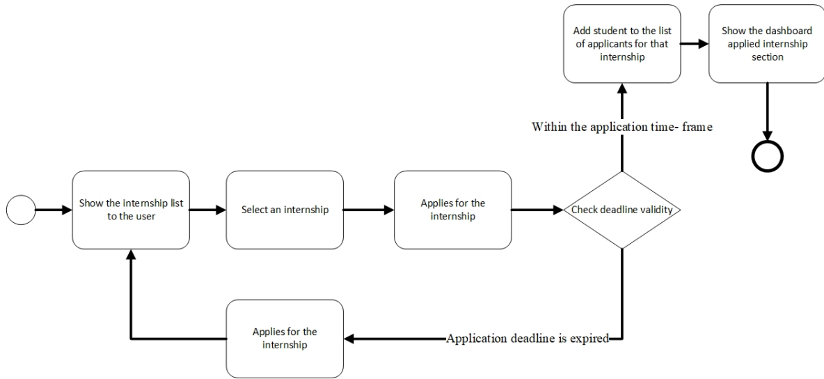
Figure 5: Sending Application for an Internships State Chart
