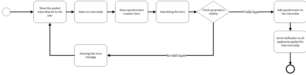
Figure 8: Creating a Questionnaire by a Company State Chart
