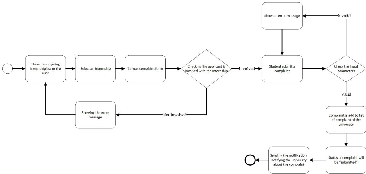
Figure 12: Submitting an Complaint by a Student State Chart
