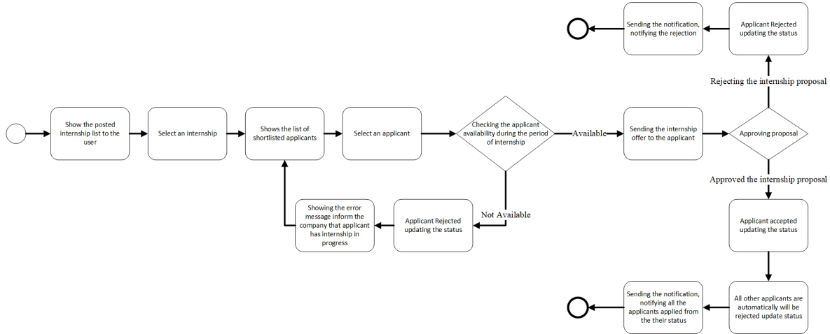
Figure 10: Making a Final Decision by a Company State Chart
