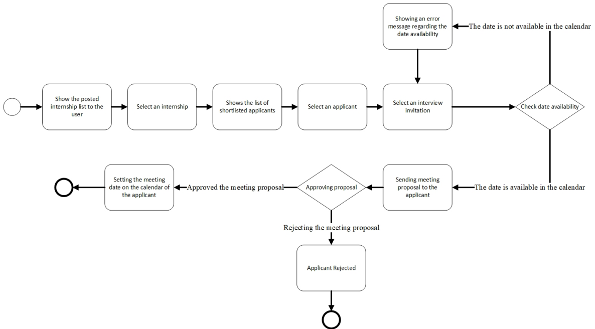
Figure 7: Scheduling Interview by a Company State Chart
