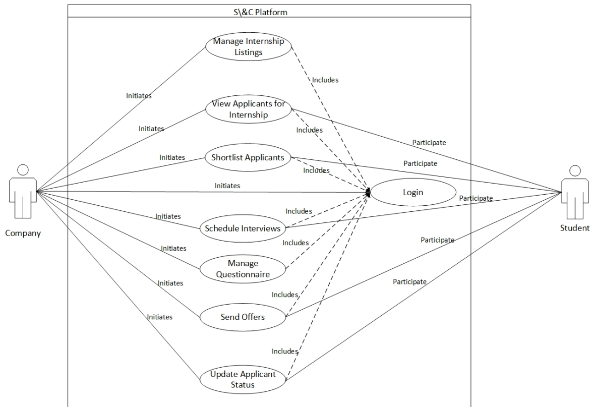
Figure 17: Use Cases Diagram for Company
