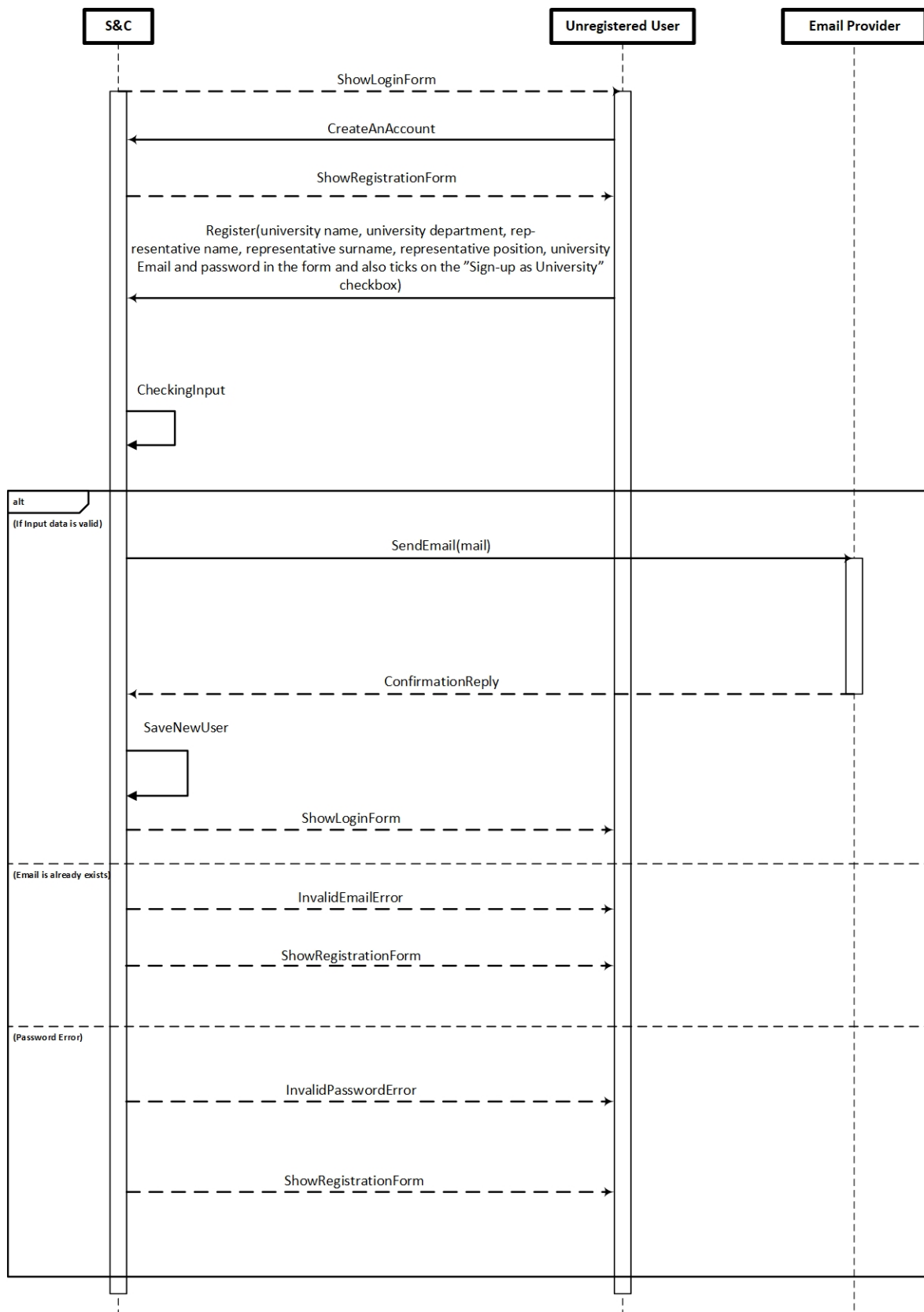
Figure 21: Registration as University Sequence Diagram
