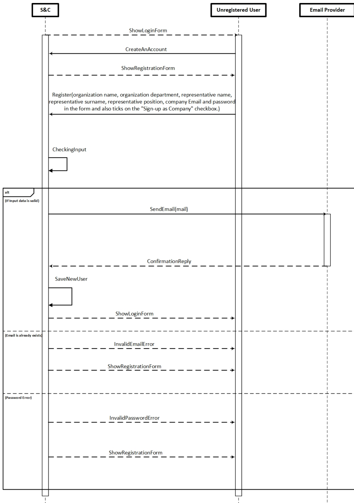
Figure 20: Registration as Company Sequence Diagram
