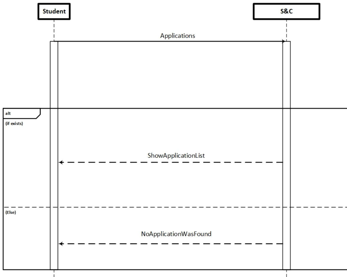
Figure 26: Track Applications Sequence Diagram
