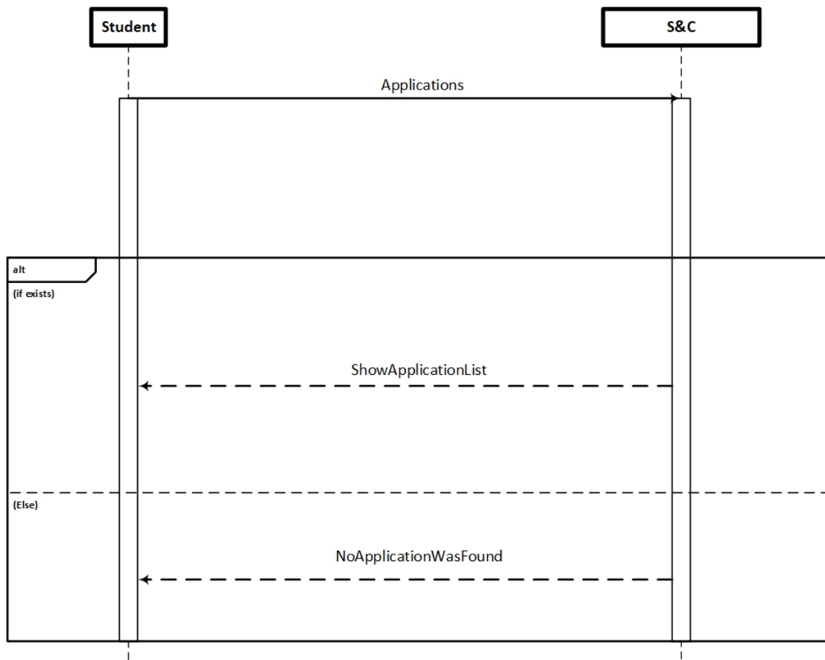
Figure 26: Student Track Applications Sequence Diagram
