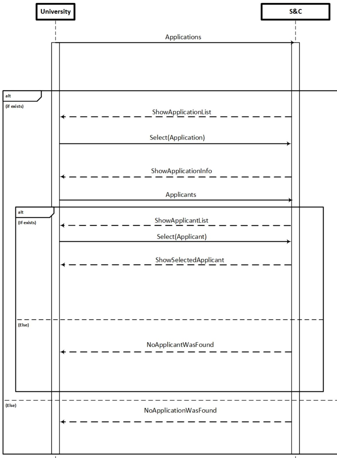
Figure 38: University Track Application Sequence Diagram
