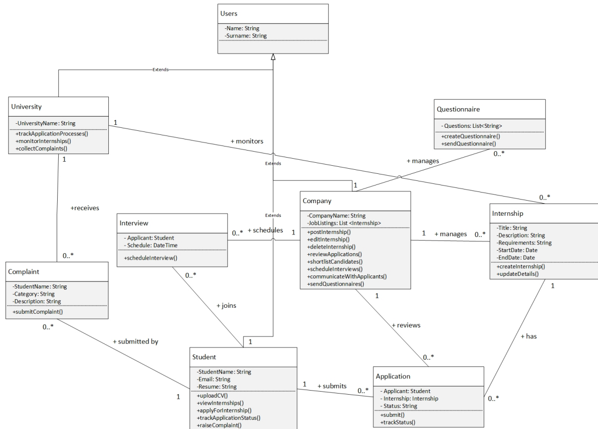
Figure 1: Class Diagram
