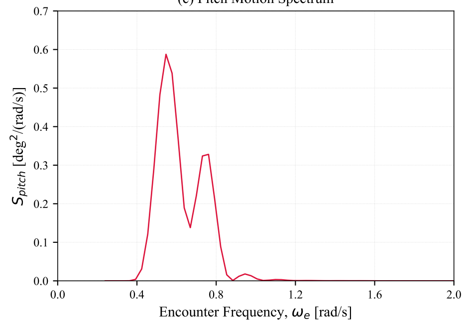
(c) Pitch Motion Spectrum
