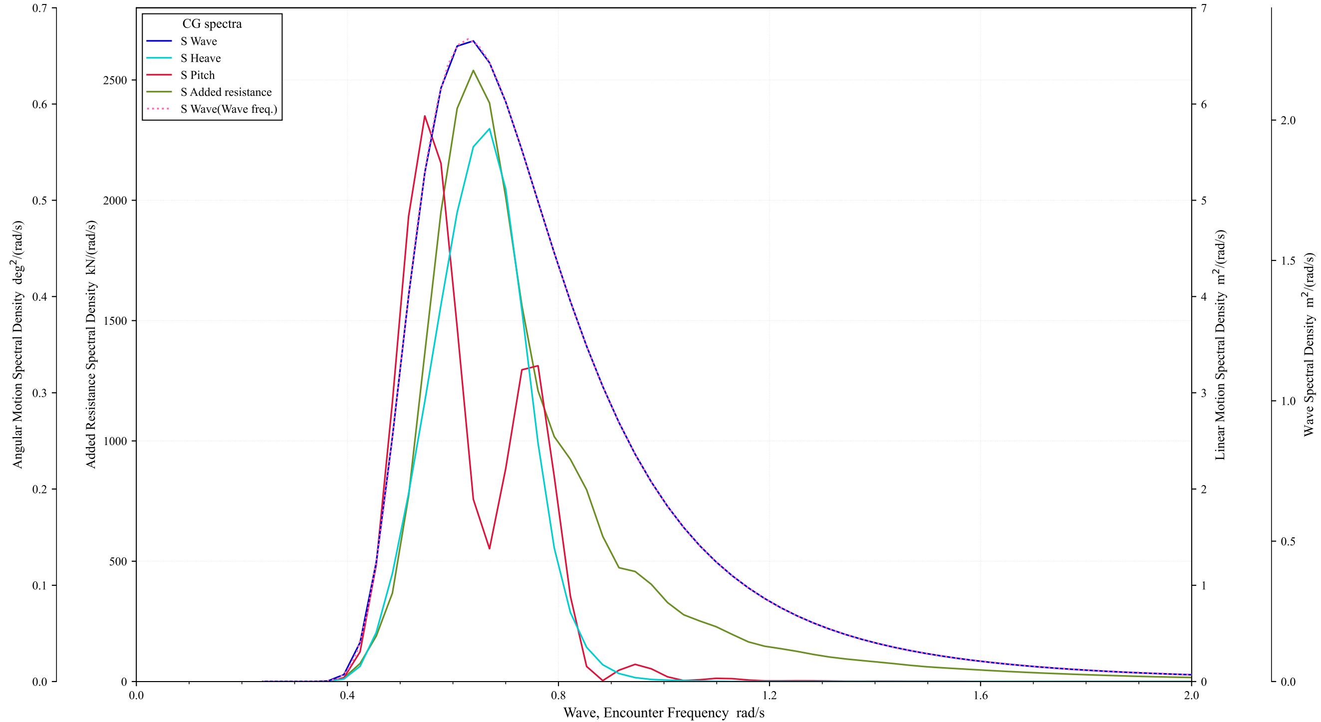
CG Motion Response Spectra
