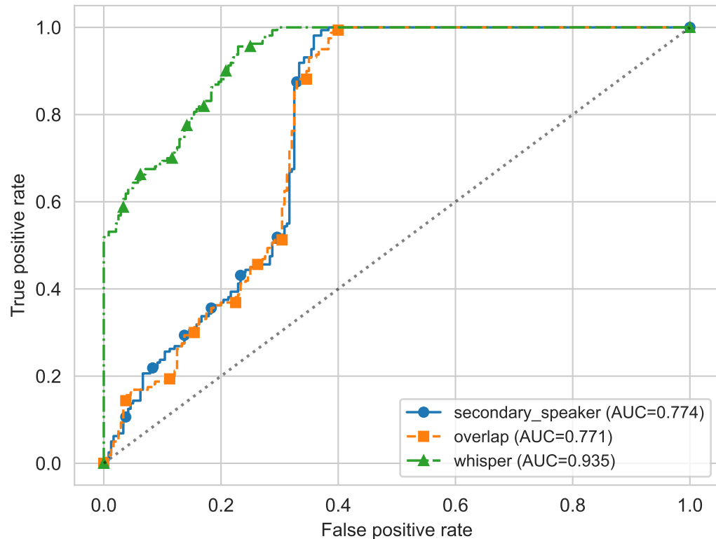
ROC – content-free acoustic anomaly
