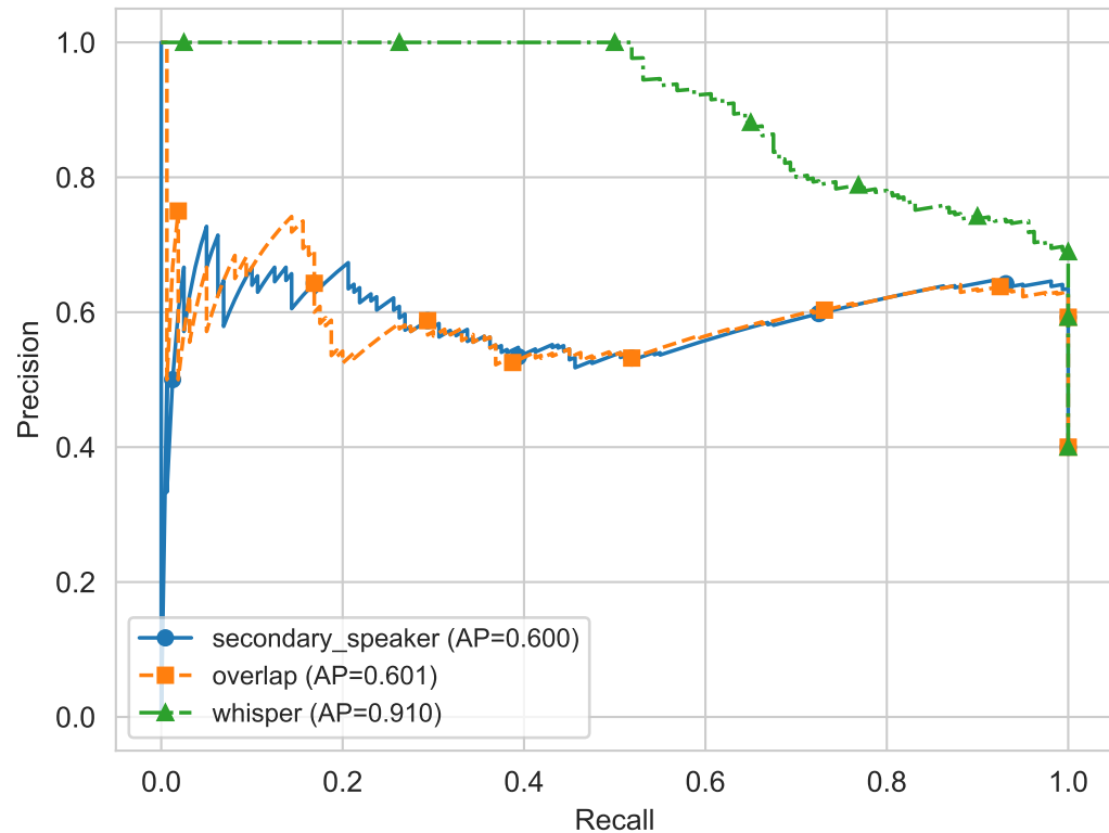
PR – content-free acoustic anomaly
