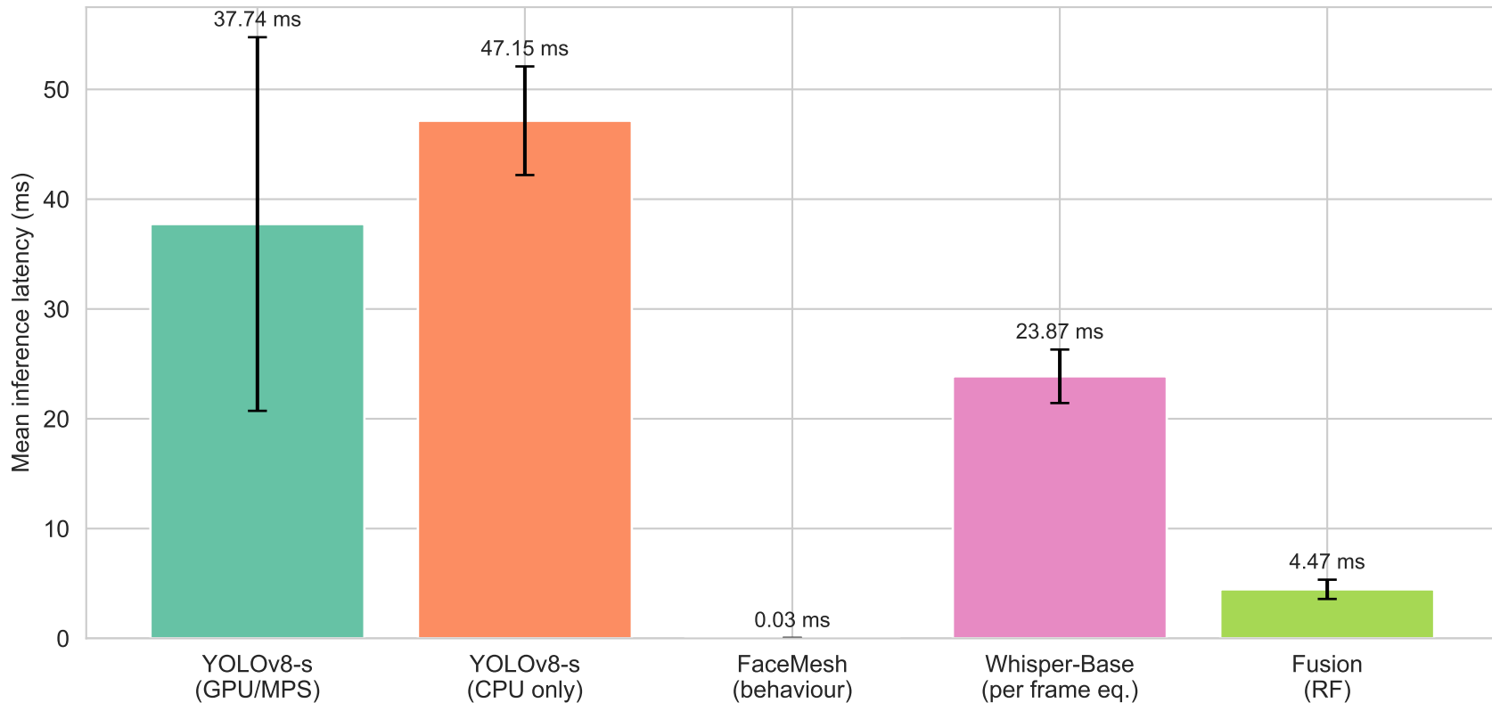
Per-module inference latency on Apple M4 Max
