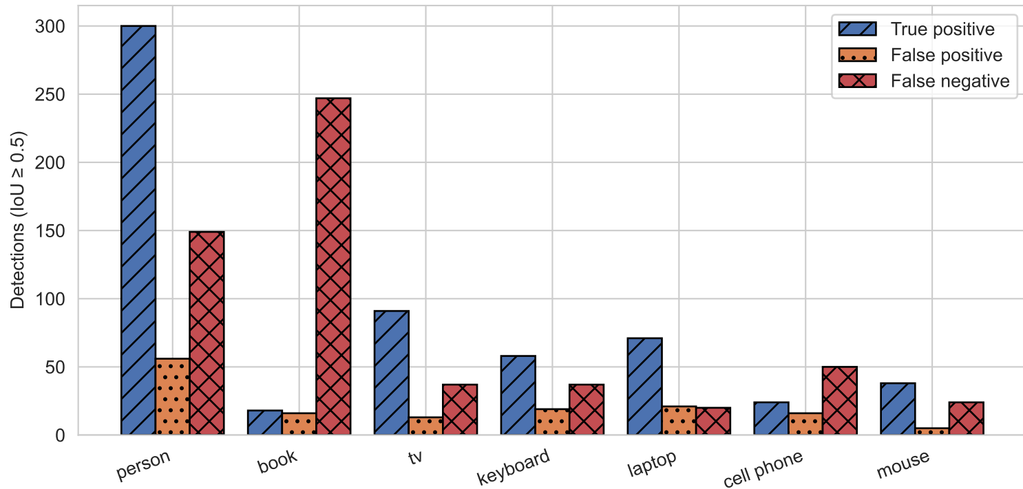
Per-class TP / FP / FN after greedy IoU matching
