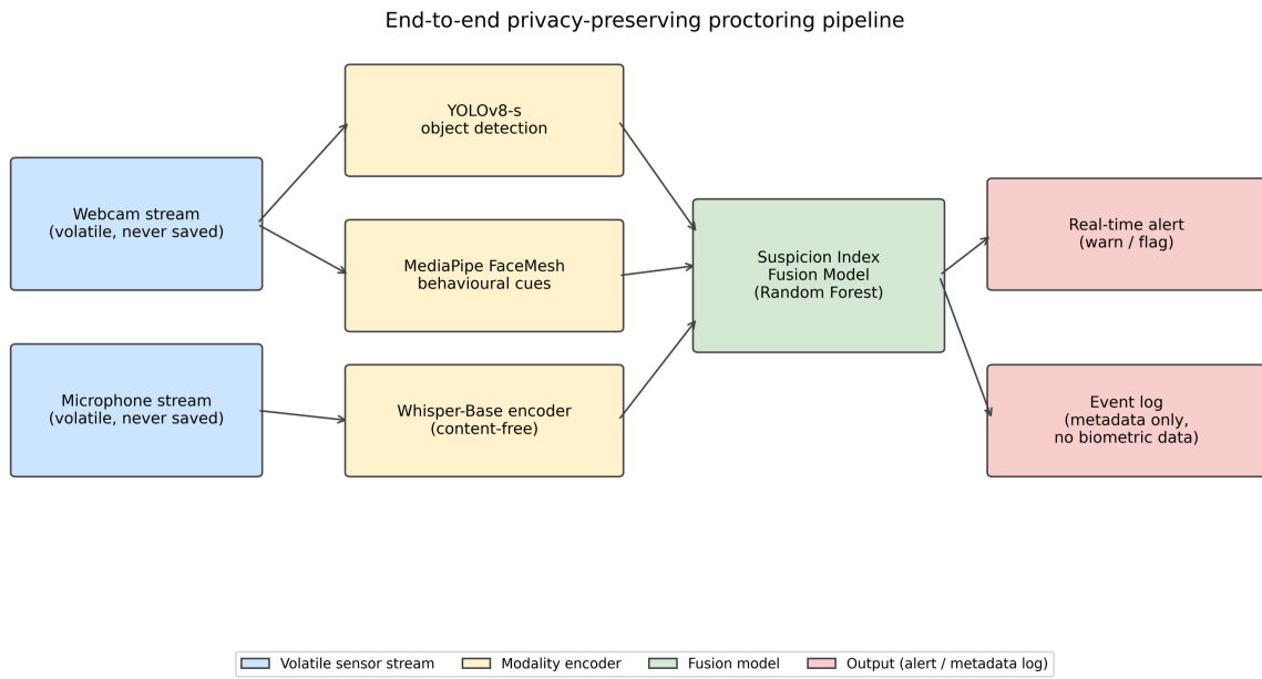
Figure 1: End-to-end privacy-preserving proctoring pipeline.
