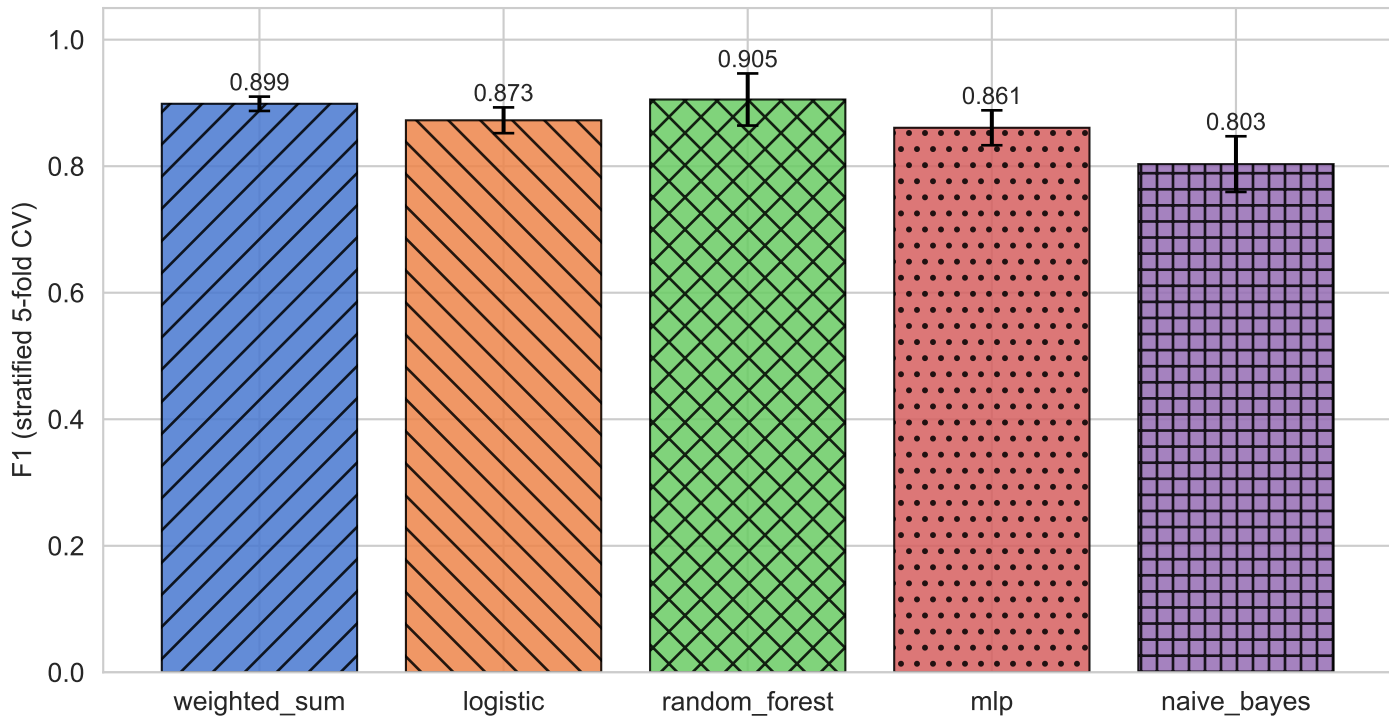
Fusion strategy comparison
