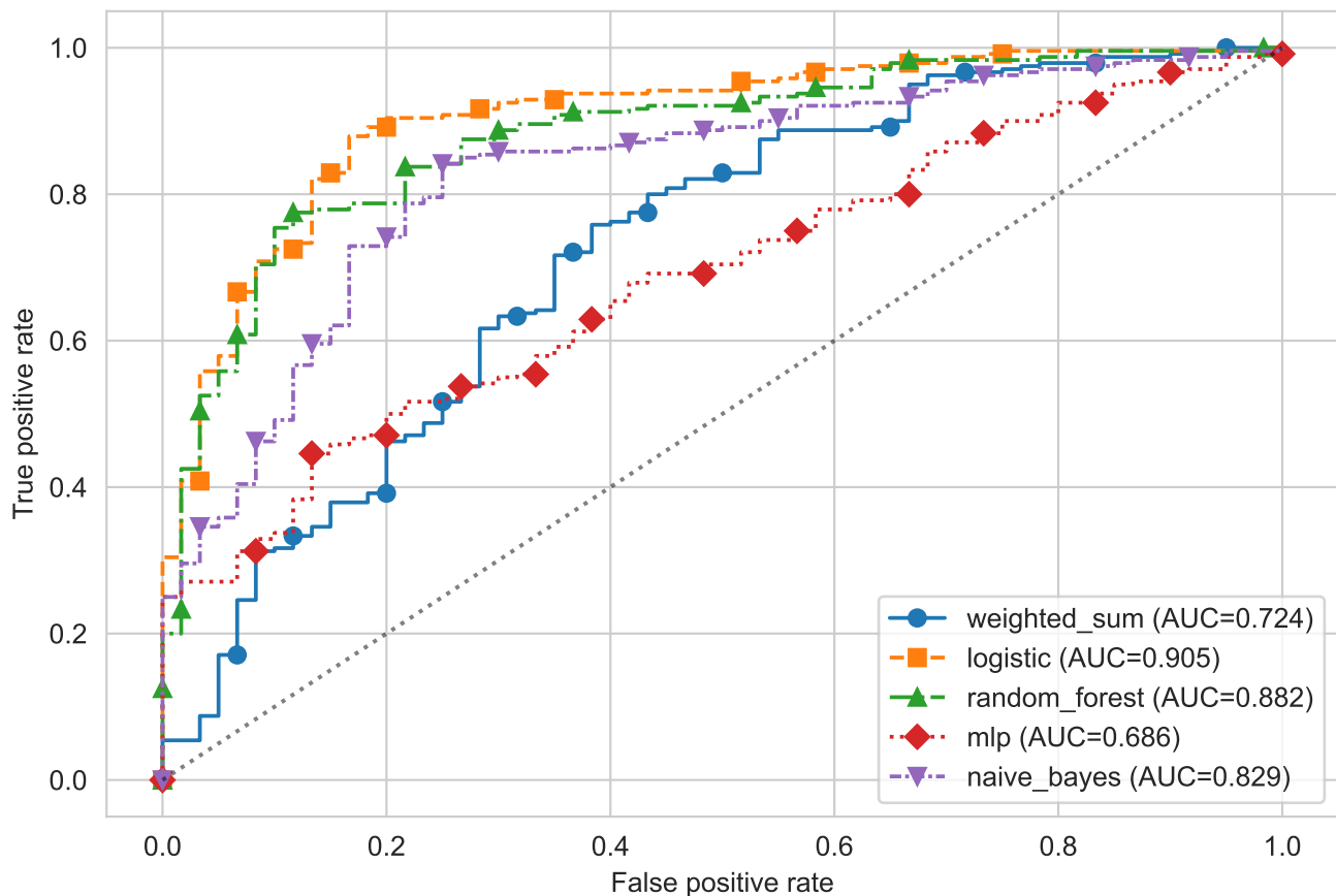
Fusion model ROC curves on stratified 5-fold CV
