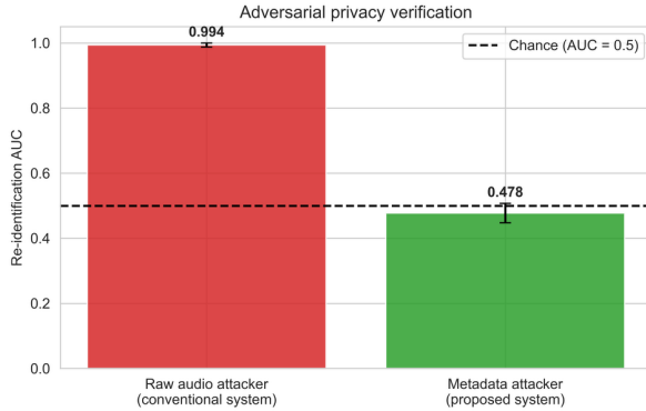
Figure 14: Adversarial privacy verification on 30 real LibriSpeech speakers: re-identification AUC achieved by a raw-audio attacker (proxy of conventional proctoring) versus a metadata-only attacker (the proposed system).
