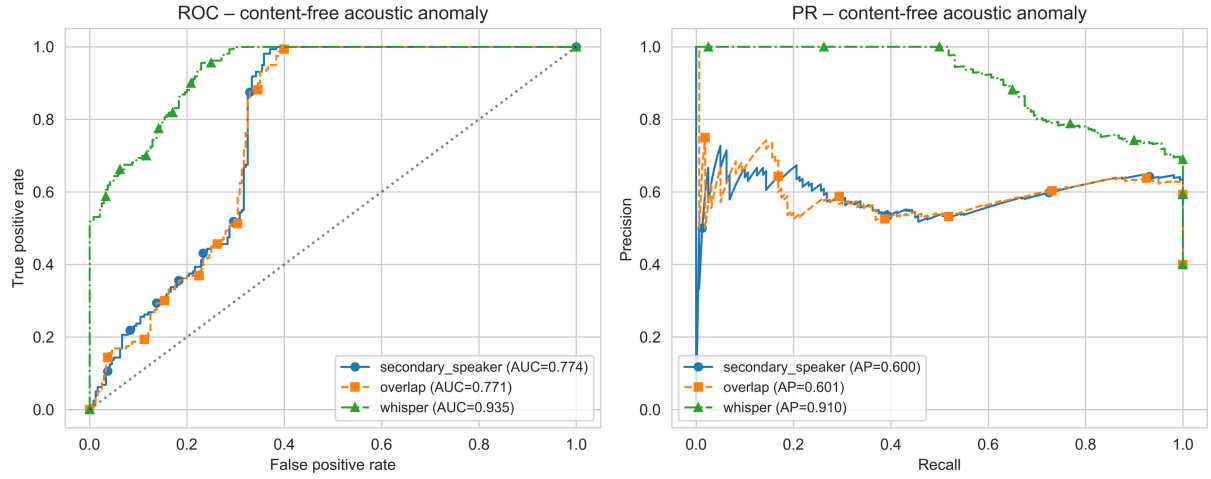
Figure 5: ROC and PR curves for the Whisper-Base content-free acoustic module on the LibriSpeech-derived benchmark.
