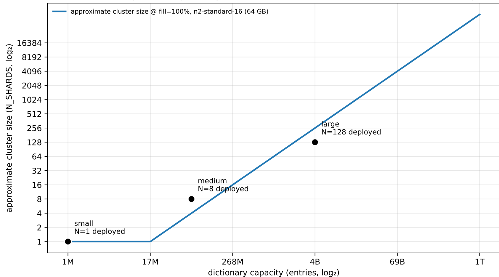
Approximate cluster size at fill=100% on n2-standard-16 (64 GB) (model: ~1.95 GB peak RSS per 1M per-shard entries, derived from v16 medium watchdog data)
