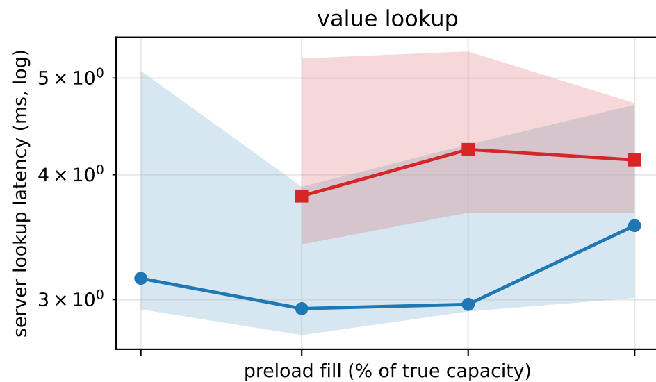
Server-side lookup latency vs. preload (p50, shaded = p10-p90)
