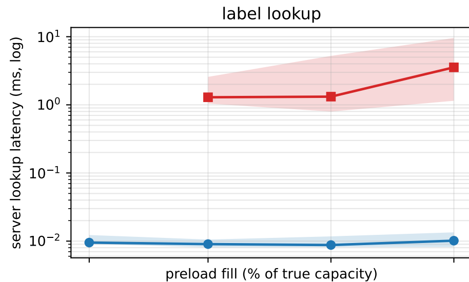
Server-side lookup latency vs. preload (p50, shaded = p10-p90)
