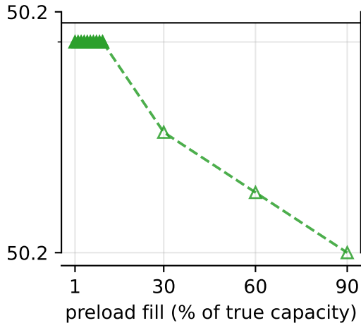
median audit proof size (KB)
