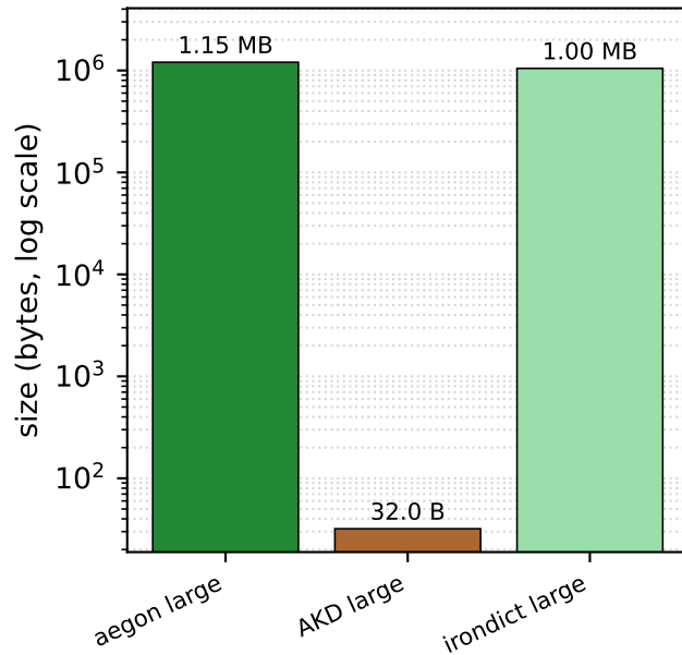
Verifier key
