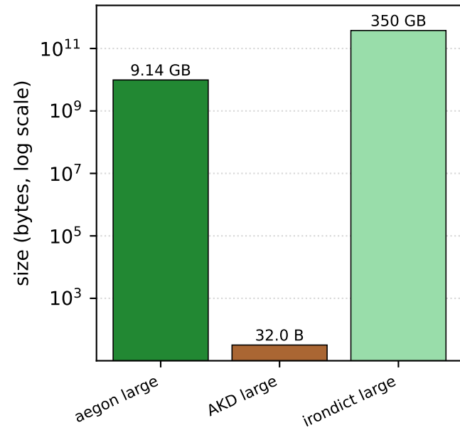
Prover key
