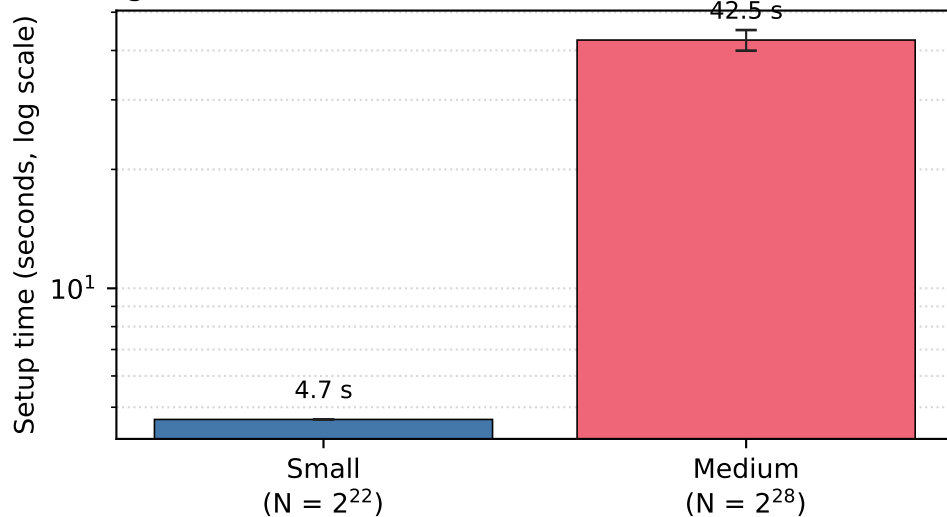
KZH-k SRS generation time (median; whiskers = min..max across shards)
