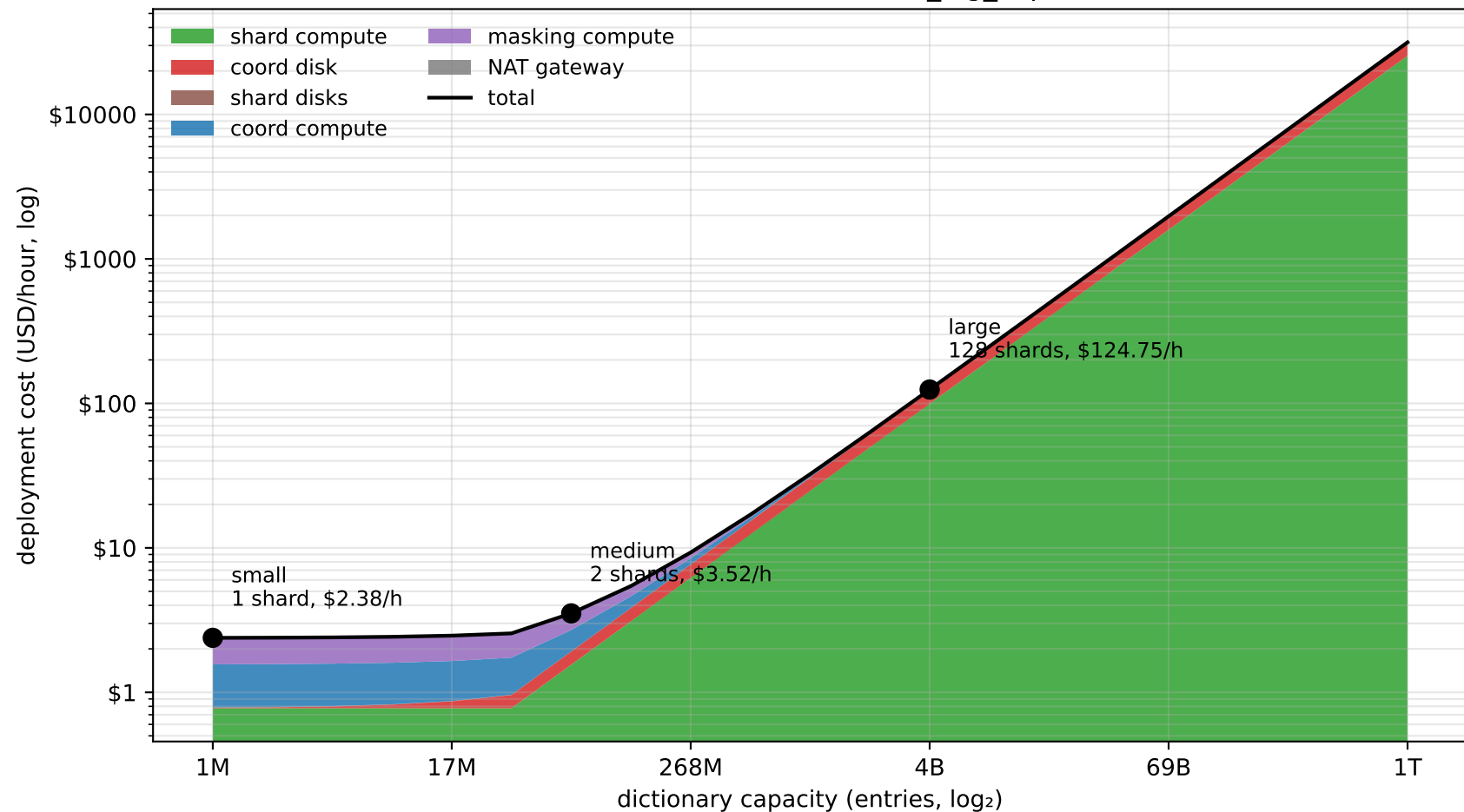
Aegon cluster cost vs. dictionary capacity (shard=n2-standard-16, coord=n2-standard-16, shard_log_cap=27, disk sized for 100% fill)
